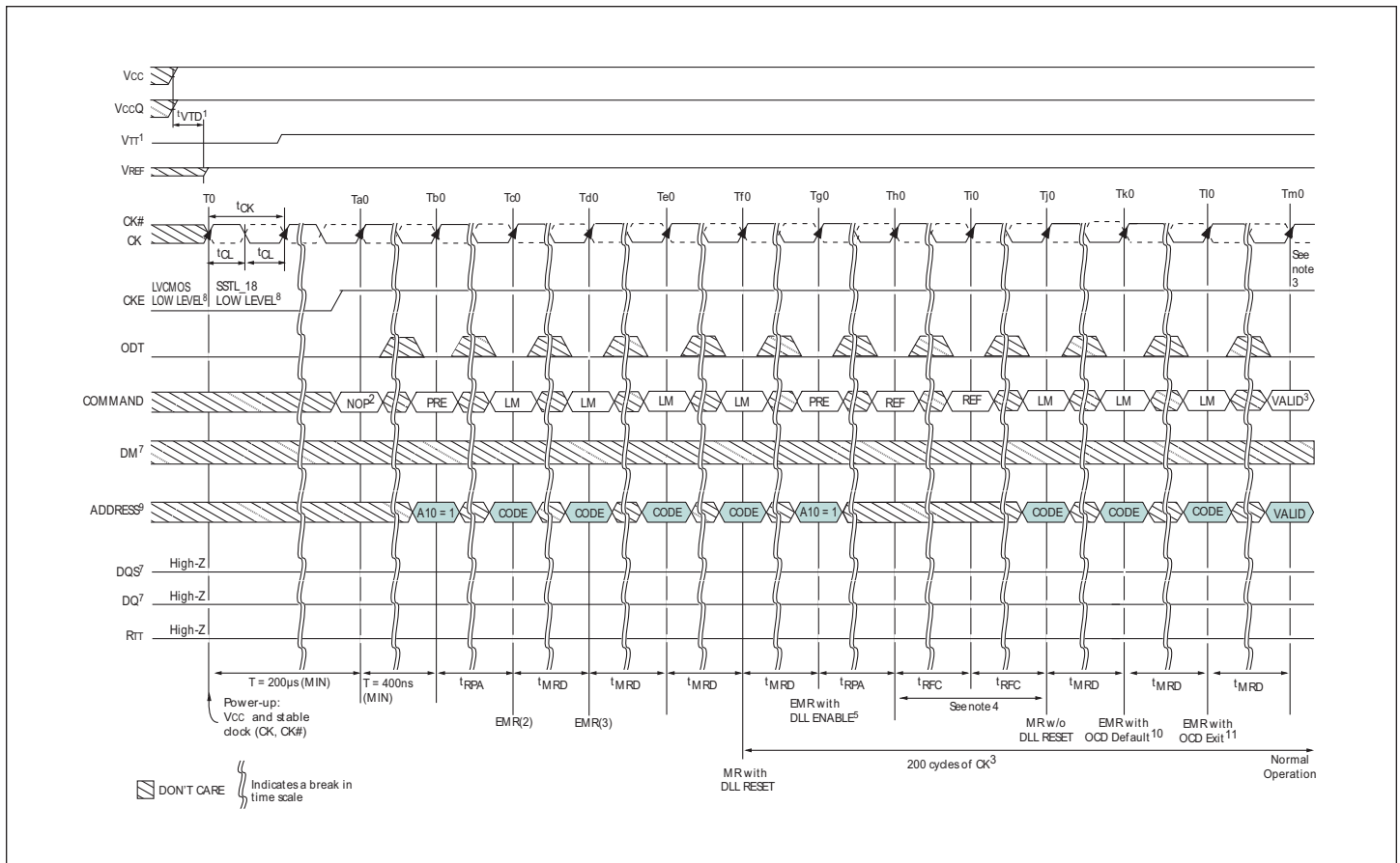
FIGURE 4 – POWER-UP AND INITIALIZATION
