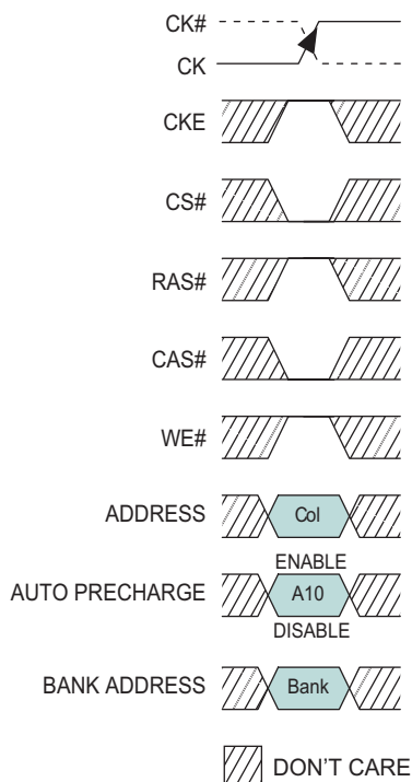
FIGURE 12 – WRITE COMMAND
