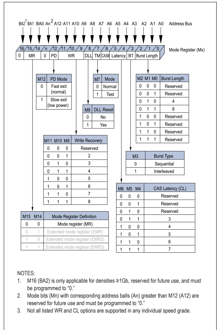
FIGURE 5 – MODE REGISTER (MR) DEFINITION
