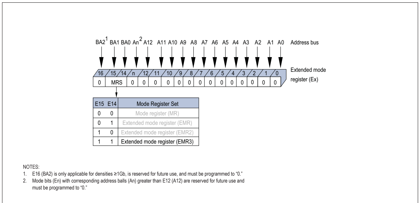
FIGURE 9 – EXTENDED MODE REGISTER 3 (EMR3) DEFINITION
