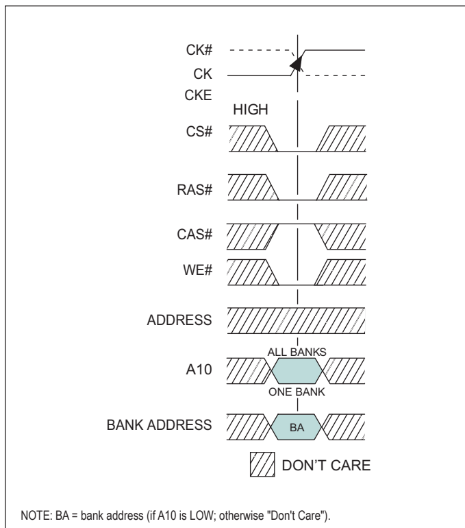
FIGURE 13 – PRECHARGE COMMAND
