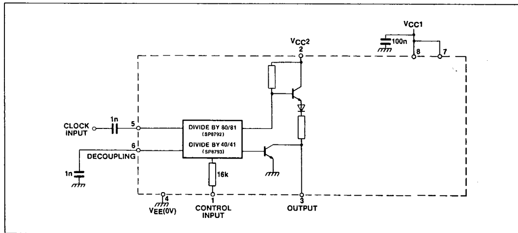
Fig. 2 Functional diagram
