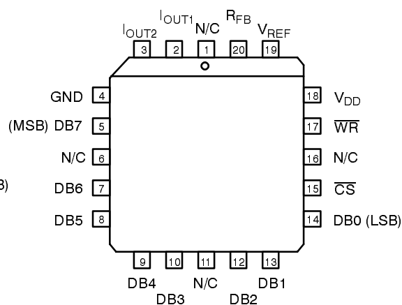
20 Pin PLCC
