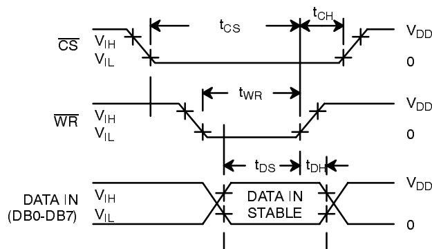
Figure 1. Write Cycle Timing Diagram
