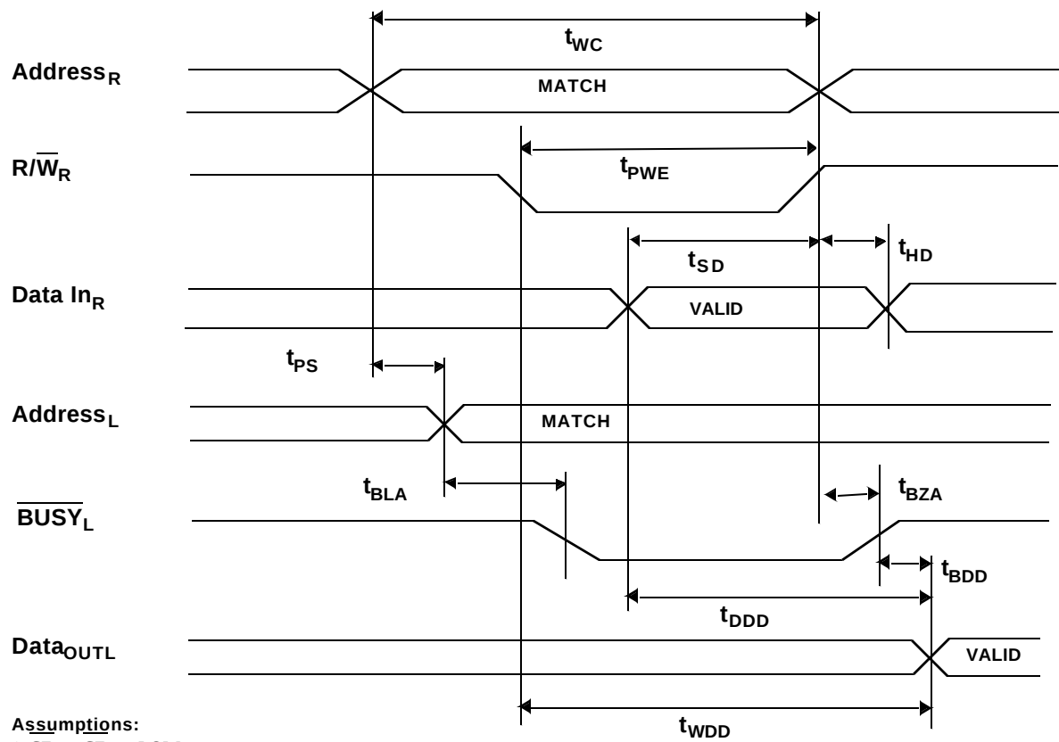
Figure 5a. Read Timing with \overline{\text{BUSY}} ( M/\overline{S}=\text{HIGH} )
