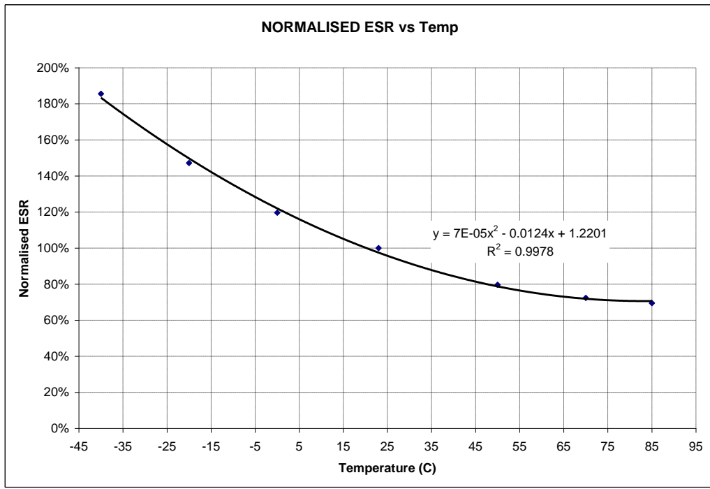
Figure 6: Normalised ESR at different temperatures
