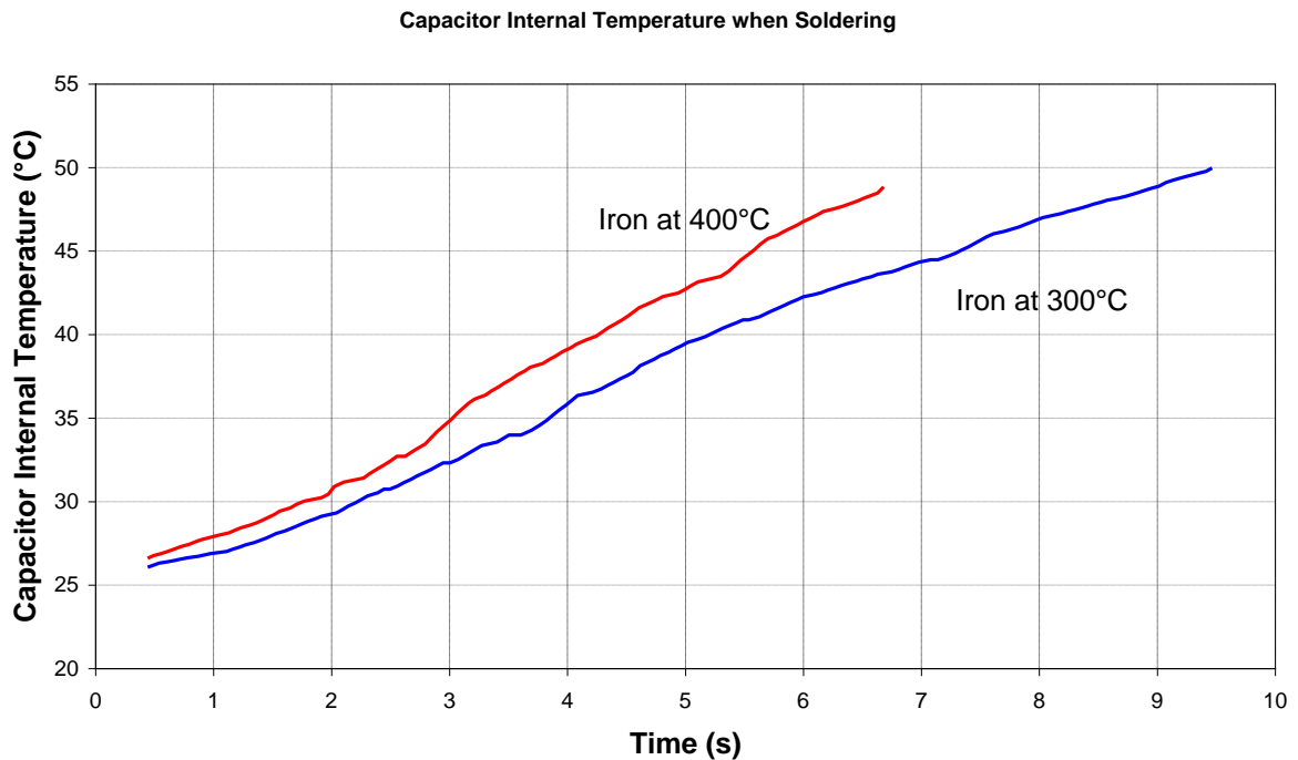
Figure 12: Capacitor temperature rise when soldering
