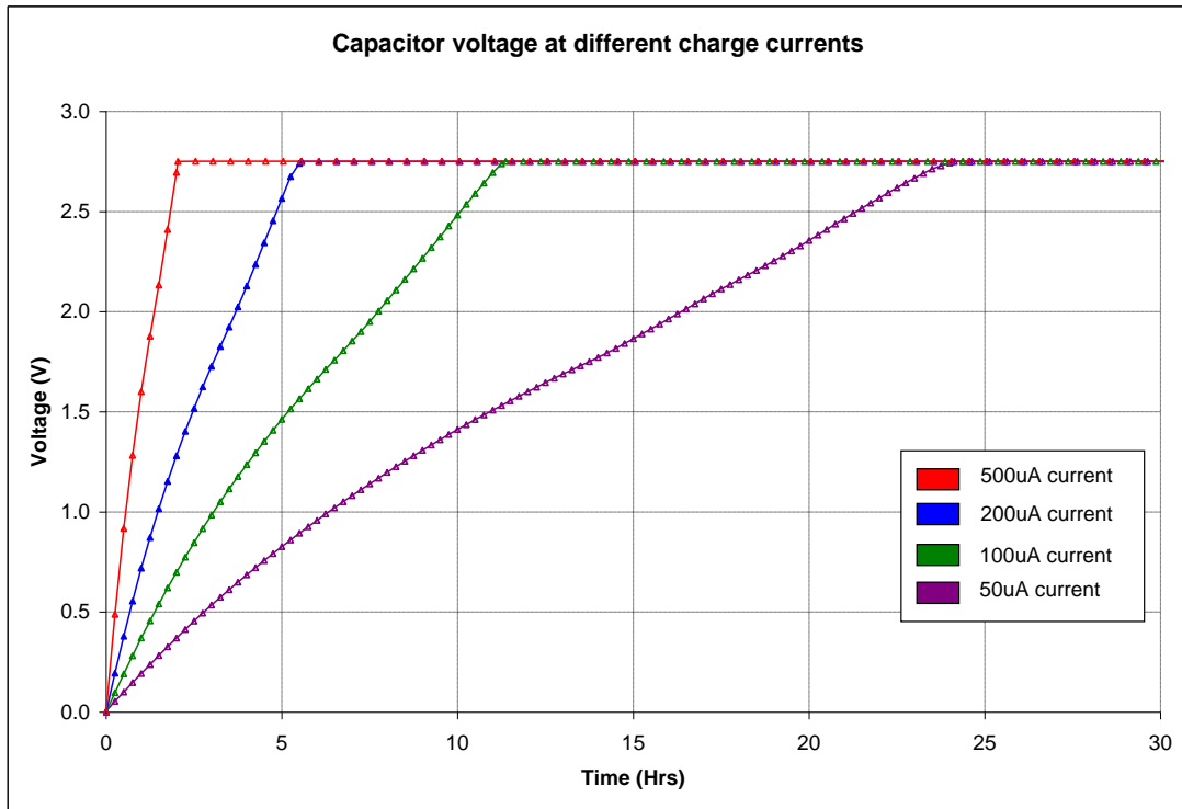
Figure 111: Voltage vs. Time for 50µA, 100µA, 200µA, 500µA charging currents at 23C
