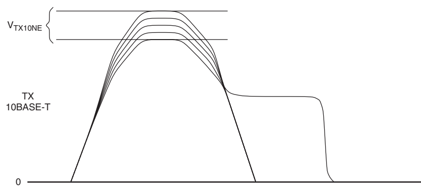
Figure 12. 10BASE-T Waveform With 1:1 Transformer Ratio
