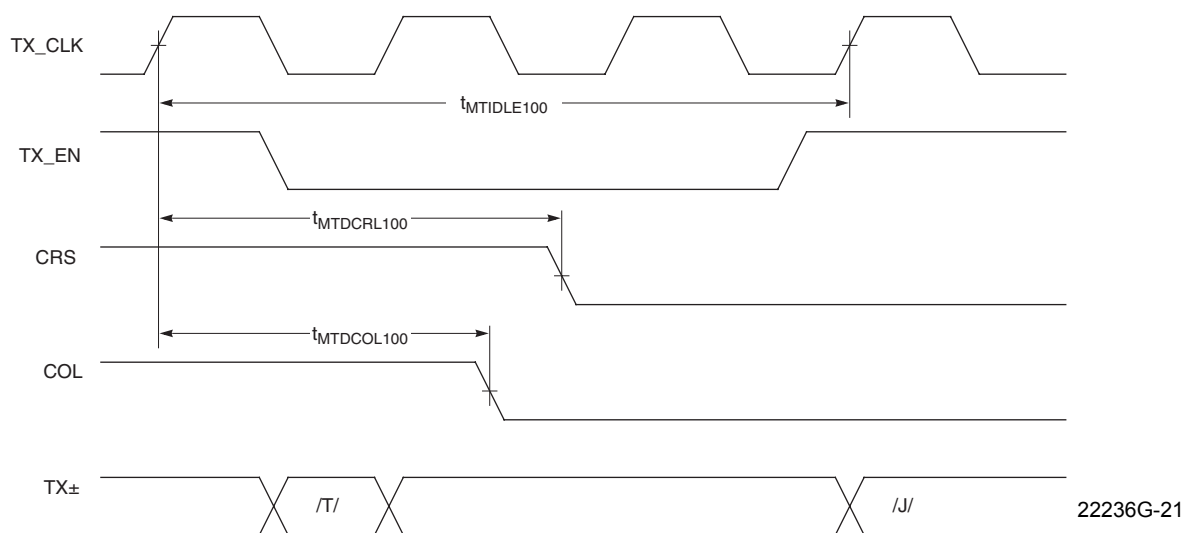
Figure 19. 100 Mbps Transmit End of Packet Timing
