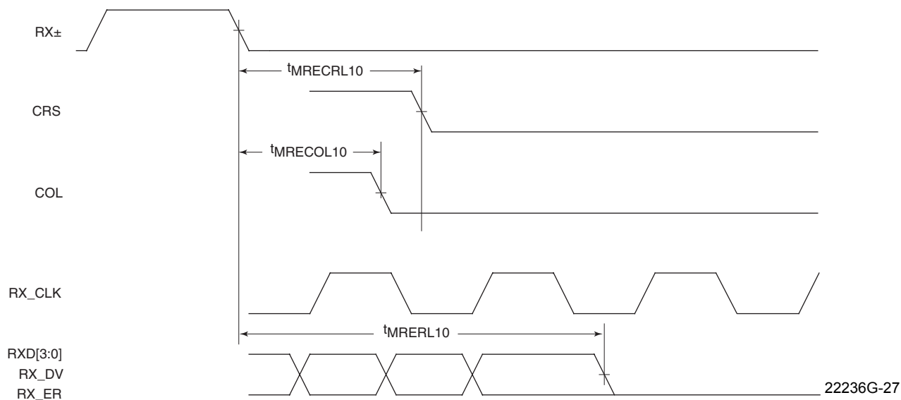
Figure 25. 10 Mbps MII Receive End of Packet Timing
