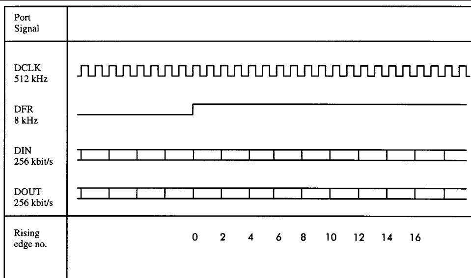
Fig.6: Timing of Data and Clocks at the GCI Interface
