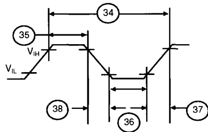
Master Clock Timing
