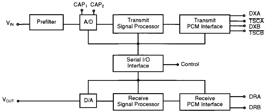
Figure 2. SLAC Device Block Diagram
