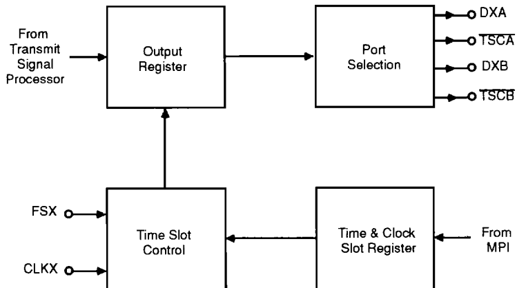
Figure 4. Transmit PCM Interface
