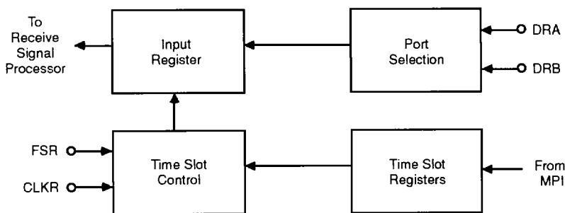
Figure 6. Receive PCM Interface
