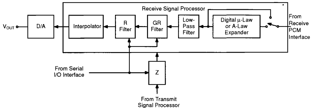
Figure 8. Receive Signal Processor
