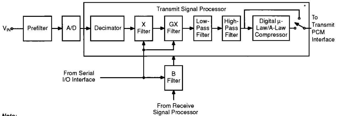
Figure 3. Transmit Signal Processor
