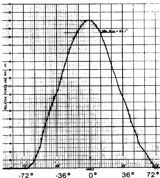
E-Plane — K-Band
