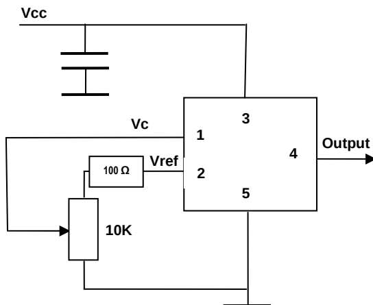
Pin Connections
