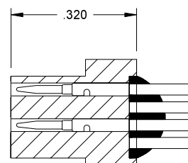
PLUG
