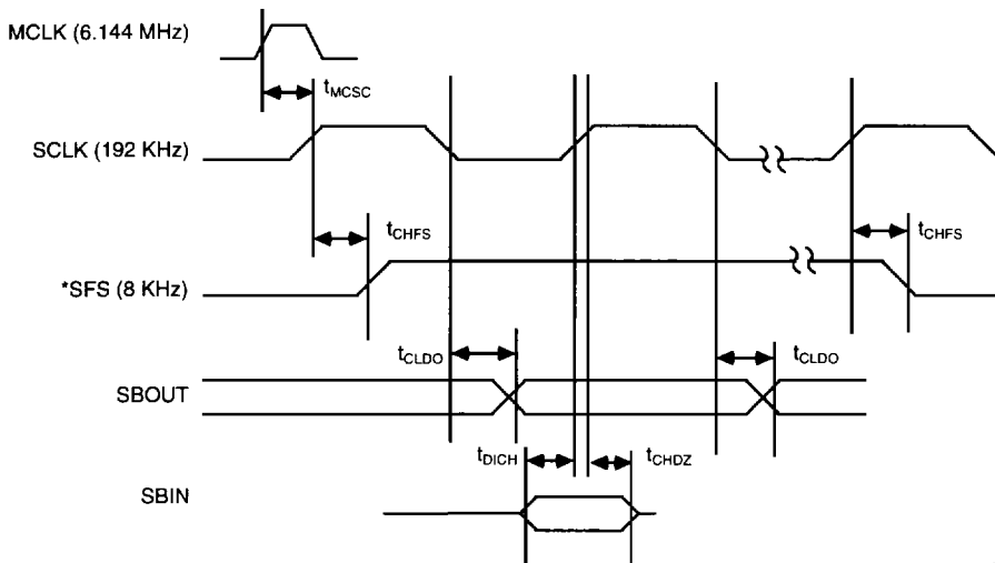
Figure 35. SBP Mode Timing
