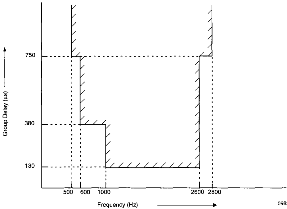
Figure 18. Group Delay Variation with Frequency (Transmit)
