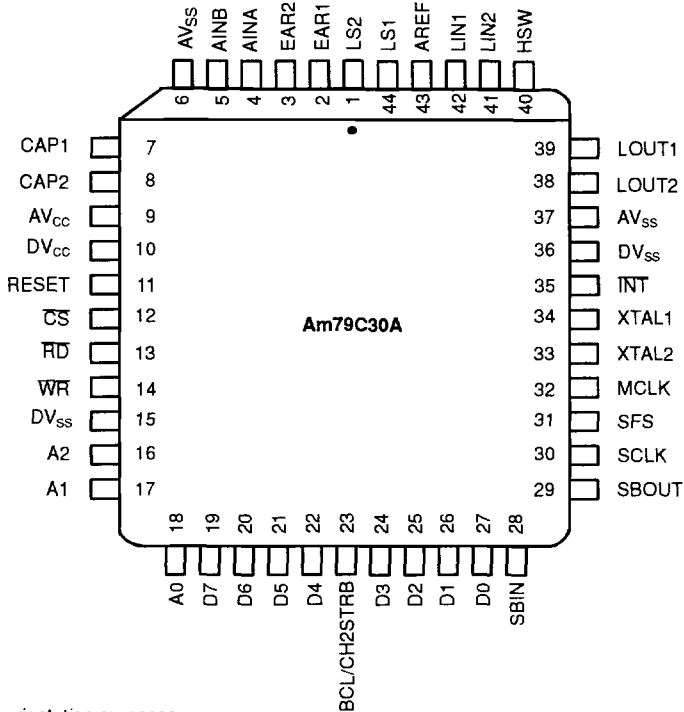
44-Pin PLCC
