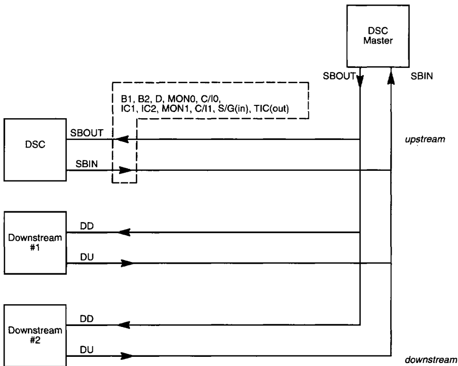
Figure 10. IOM-2 Slave Mode Operation without Bus Reversal
