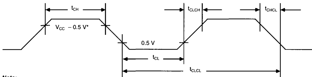
Figure 33. External Clock Driver (XTAL2) Timing
