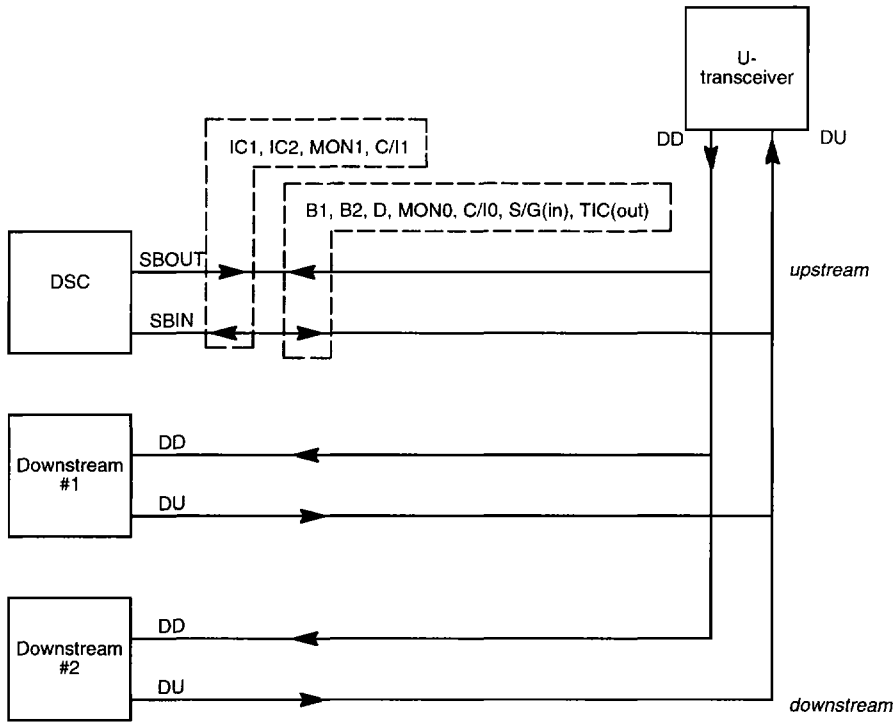
Figure 9. IOM-2 Slave Mode Operation with Bus Reversal
