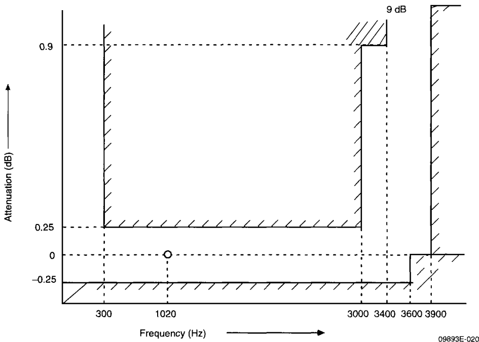
Figure 21. Attenuation/Frequency Distortion (Receive)
