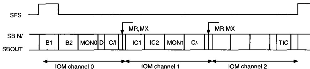
Figure 6. IOM-2 Terminal Mode Frame Structure
