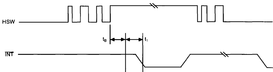
Figure 32. Hookswitch Debounce Timing
