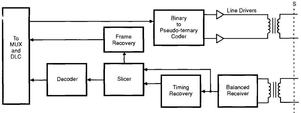
Figure 1. LIU Block Diagram
