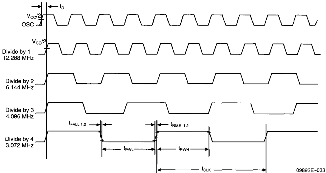
Figure 34. OSC/MCLK Timing
