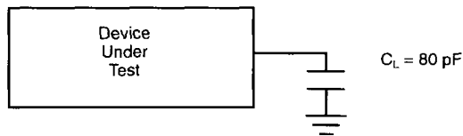
Figure 39. Switching Test Load Circuit
