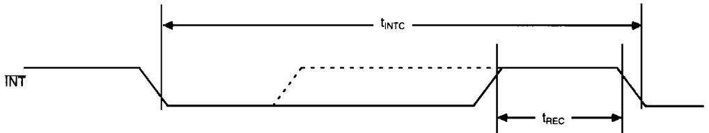
Figure 30. INT Timing
