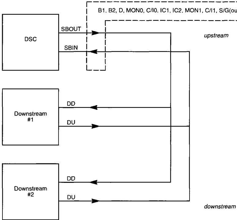
Figure 8. IOM-2 Master Mode Operation
