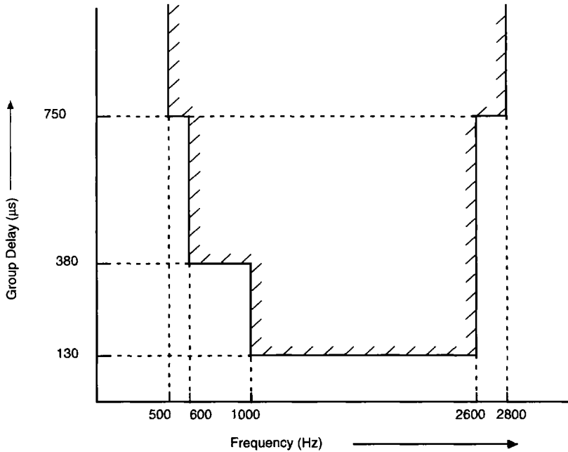
Figure 22. Group Delay Variation with Frequency (Receive)
