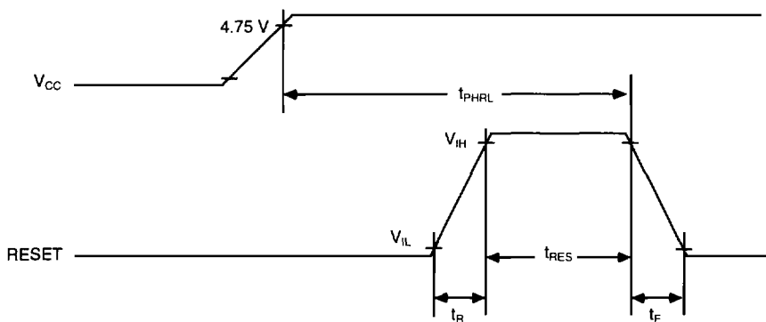
Figure 31. Reset Timing
