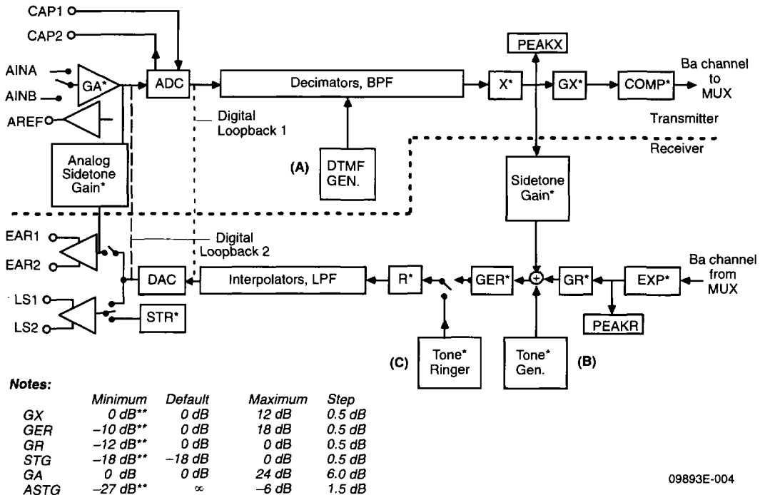
Figure 3. Main Audio Processor Block Diagram
