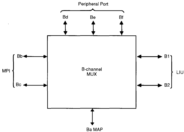
Figure 2. MUX Logical Channels
