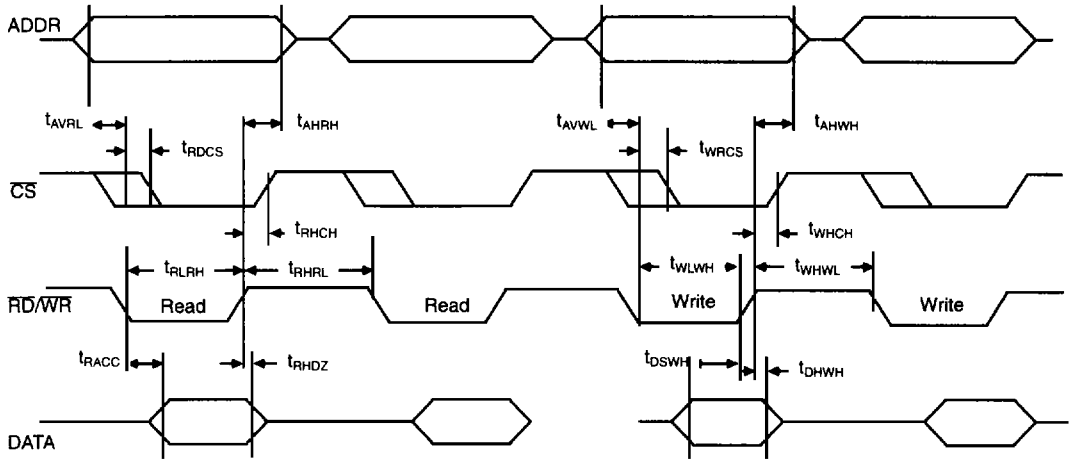
Figure 29. Microprocessor Read/Write Timing
