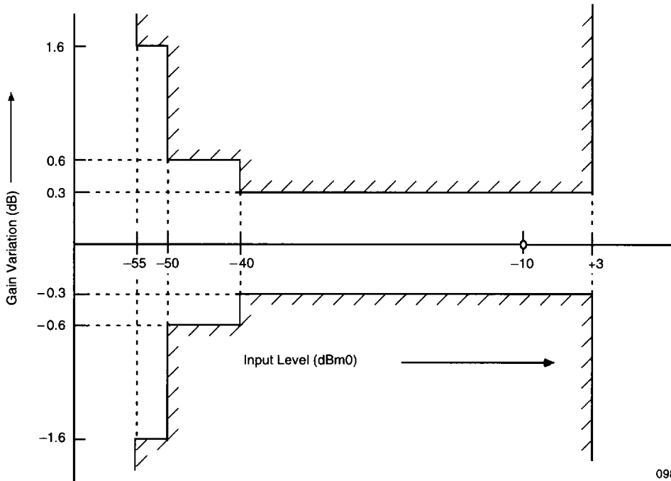
Figure 19. Gain Tracking Error (Transmit) (CCITT Method 2 at 1020 Hz)
