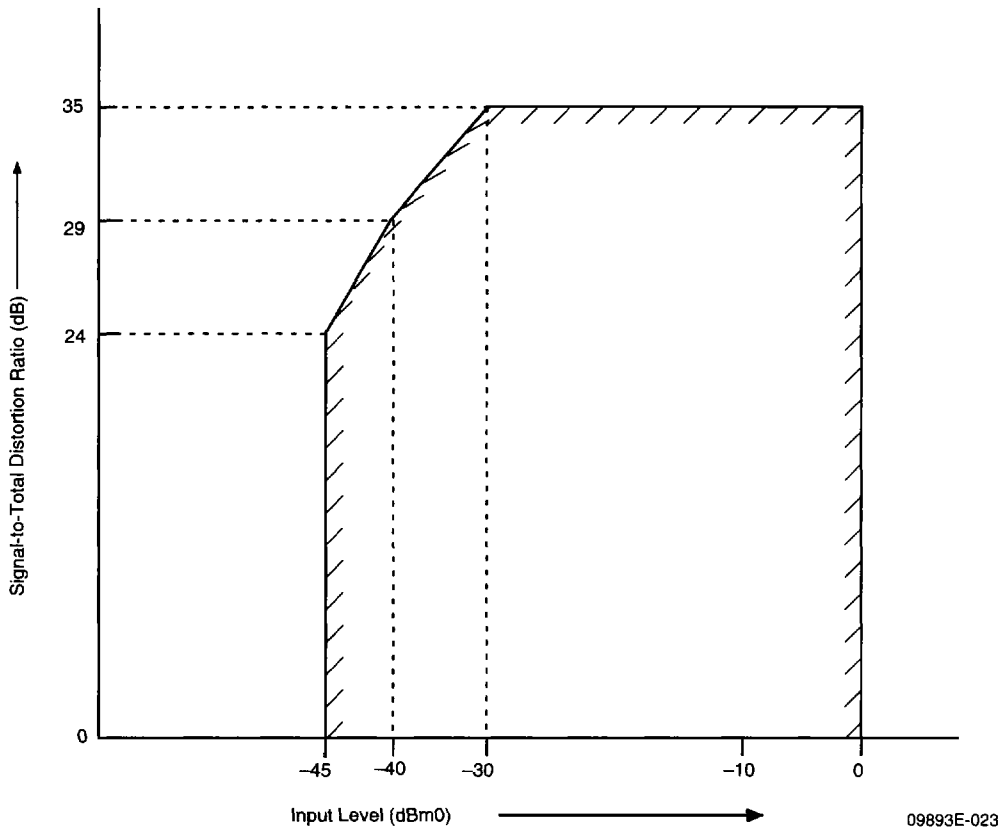
Figure 24. Signal-to-Total-Distortion Ratio (Receive) (CCITT Method 2 at 1020 Hz)
