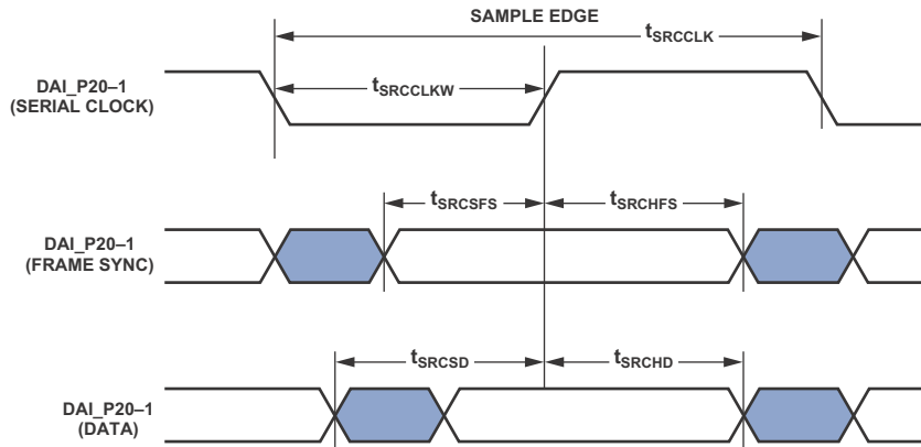
Figure 29. ASRC Serial Input Port Timing
