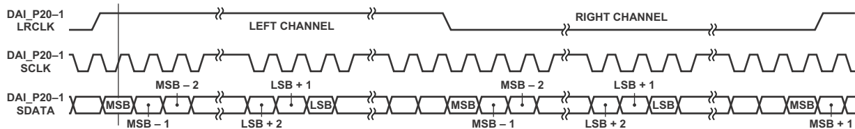
Figure 34. Left-Justified Mode
