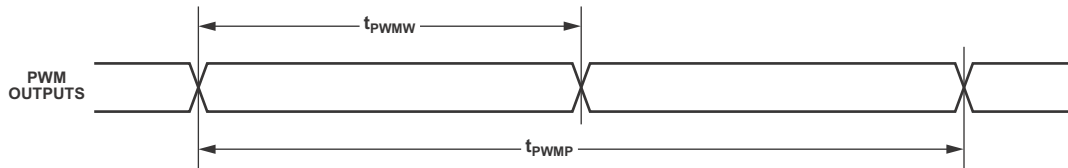
Figure 31. PWM Timing
