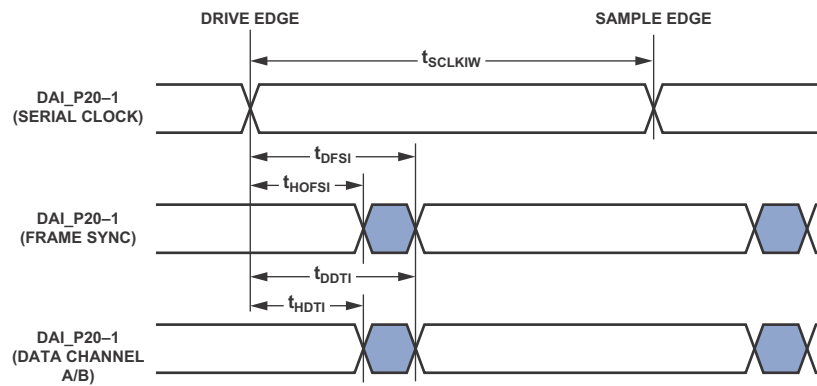
Figure 36. S/PDIF Receiver Internal Digital PLL Mode Timing
