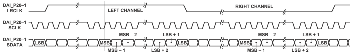
Figure 32. Right-Justified Mode
