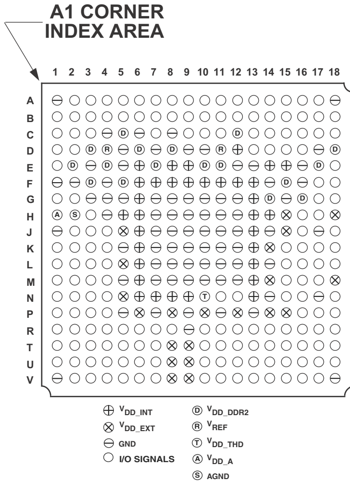
Figure 51. Ball Configuration, Automotive Pin Out
