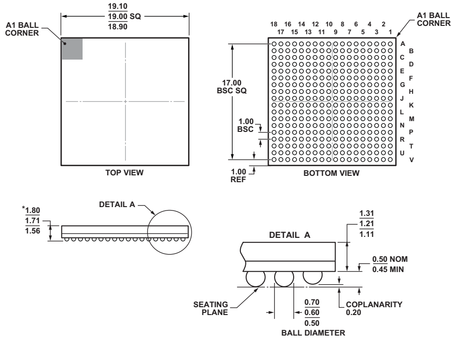
Figure 53. 324-Ball Plastic Ball Grid Array [CSP_BGA] (BC-324-1)
