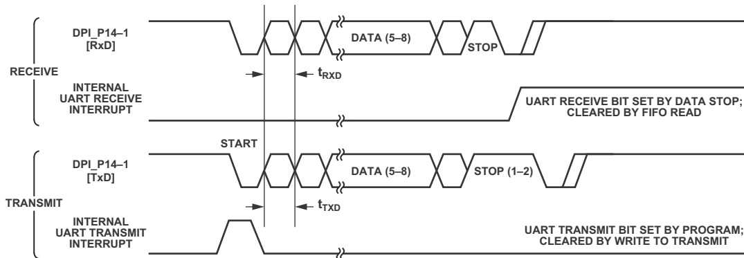
Figure 42. UART Port—Receive and Transmit Timing
