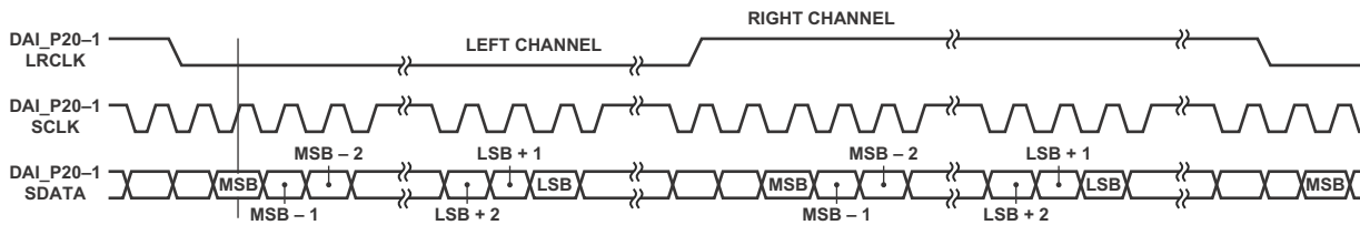
Figure 33. I 2 S-Justified Mode
