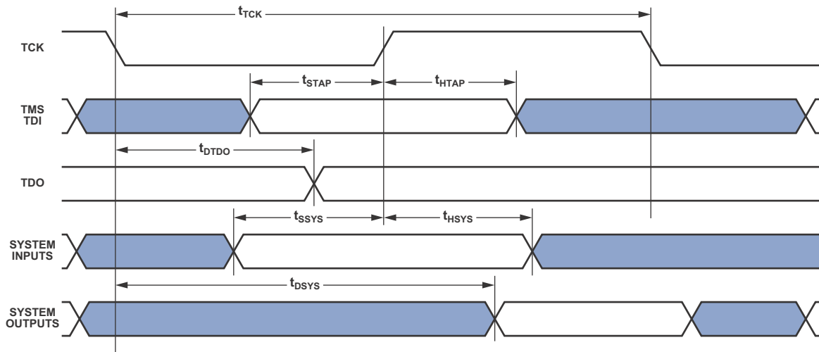
Figure 44. IEEE 1149.1 JTAG Test Access Port
