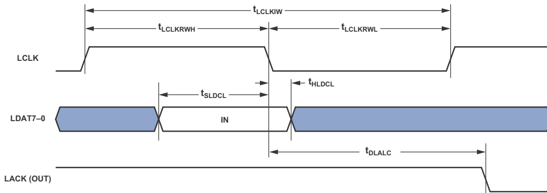
Figure 22. Link Ports—Receive
