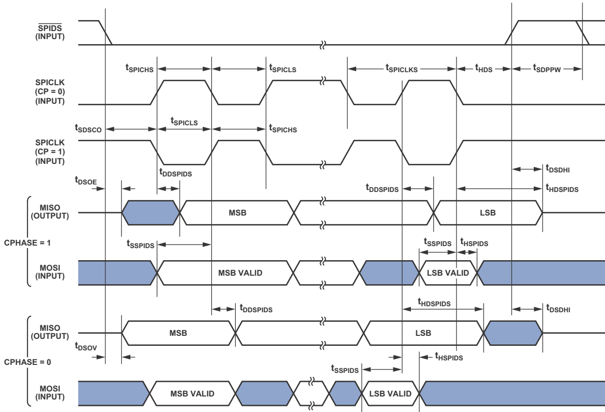
Figure 38. SPI Slave Timing
