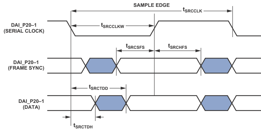
Figure 30. ASRC Serial Output Port Timing
