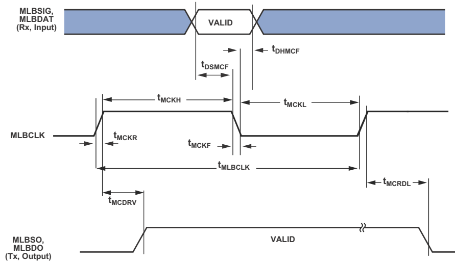
Figure 40. MLB Timing (5-Pin Interface)
