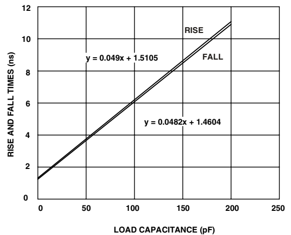
Figure 49. Typical Output Rise/Fall Time (20% to 80%, V_{DD\_EXT} = Min )
