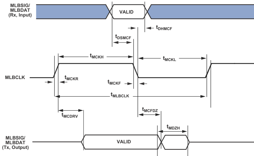
Figure 39. MLB Timing (3-Pin Interface)
