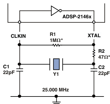
Figure 8. Recommended Circuit for Fundamental Mode Crystal Operation
