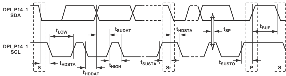
Figure 43. Fast and Standard Mode Timing on the TWI Bus
