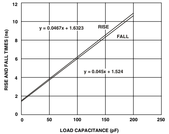
Figure 48. Typical Output Rise/Fall Time (20% to 80%, V_{DD\_EXT} = Max )
