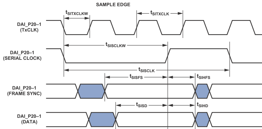
Figure 35. S/PDIF Transmitter Input Timing
