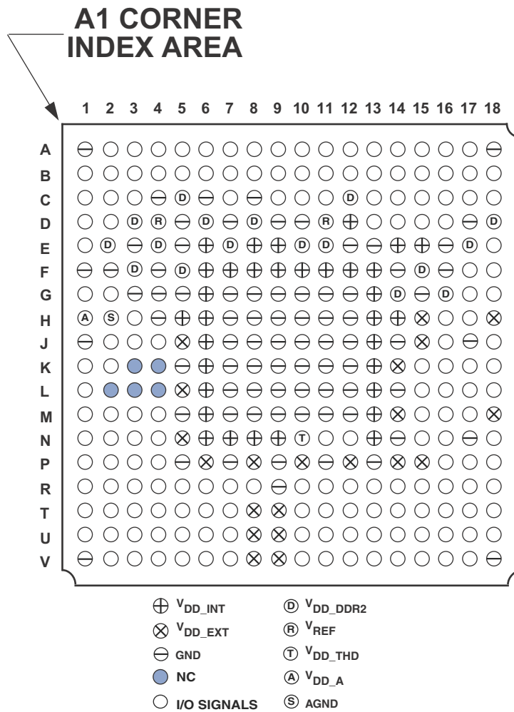
Figure 52. Ball Configuration, Standard Models
