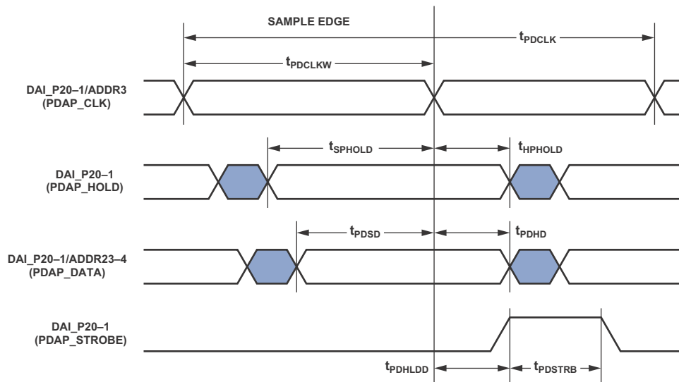
Figure 28. PDAP Timing
