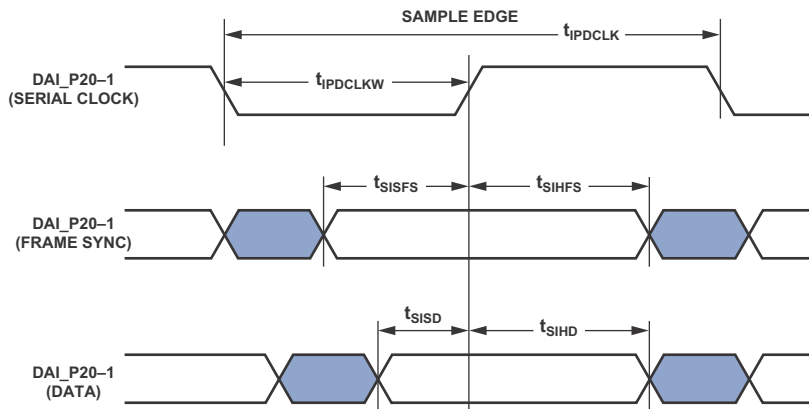
Figure 27. IDP Master Timing
