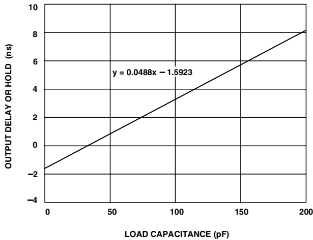
Figure 50. Typical Output Delay or Hold vs. Load Capacitance (at Ambient Temperature)
