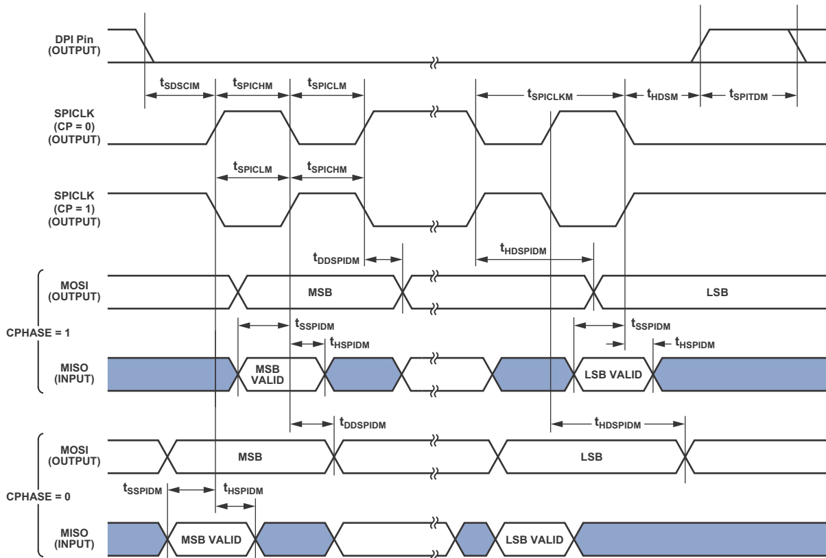
Figure 37. SPI Master Timing
