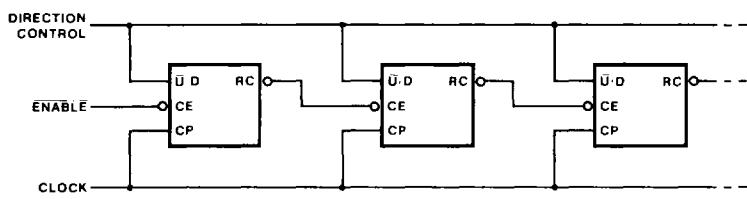
Figure c: Synchronous N-Stage Counter With Parallel Gated Carry/Borrow
