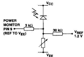
Figure 2b. Power Monitor Circuit.
