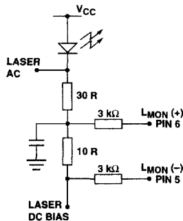
Figure 2a. Laser Bias Monitor.
