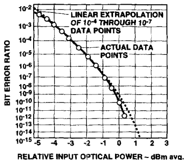
Figure 3. Relative Input Optical Power-dBm Avg.
