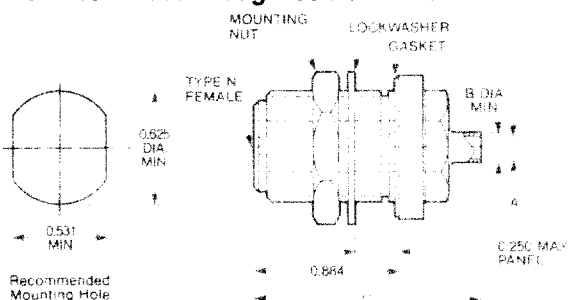
Bulkhead Feedthrough Cable Female
