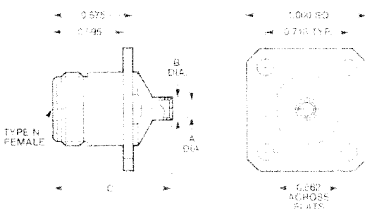
Flange Mount Cable Female
