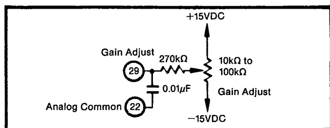
FIGURE 11. Connecting Optional Gain Adjust.
