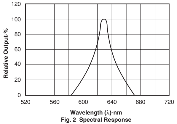
Fig. 2 Spectral Response
