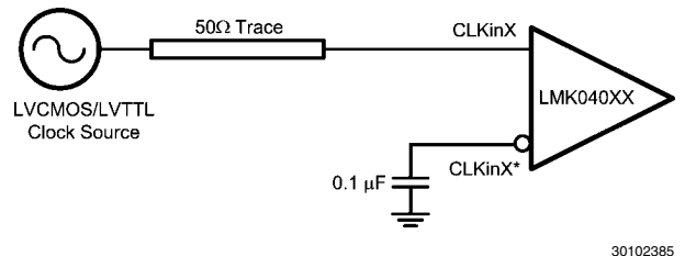
FIGURE 27. DC Coupled LVCMOS/LVTTL Reference Clock
