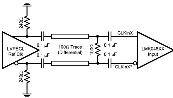
FIGURE 24. CLKin/X* Termination for an LVPECL Reference Clock Source
