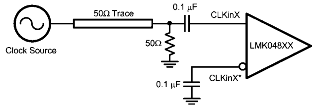
FIGURE 26. CLKin/X* Single-ended Termination
