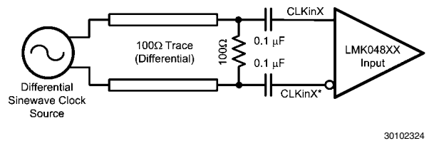
FIGURE 25. CLKin/X* Termination for a Differential Sinewave Reference Clock Source
