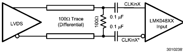
FIGURE 23. CLKin/X* Termination for an LVDS Reference Clock Source
