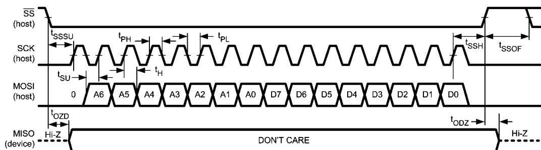
FIGURE 2. SPI Write
