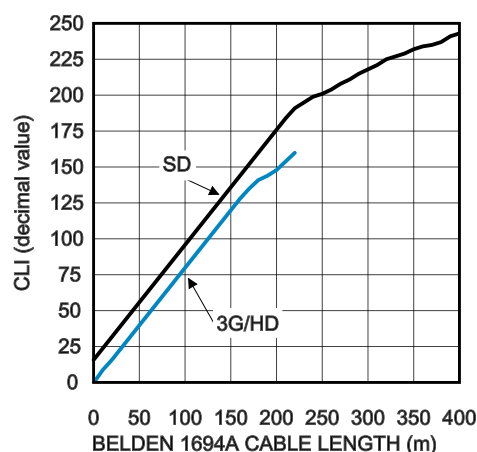
FIGURE 12. CLI vs. Belden 1694A Cable Length
