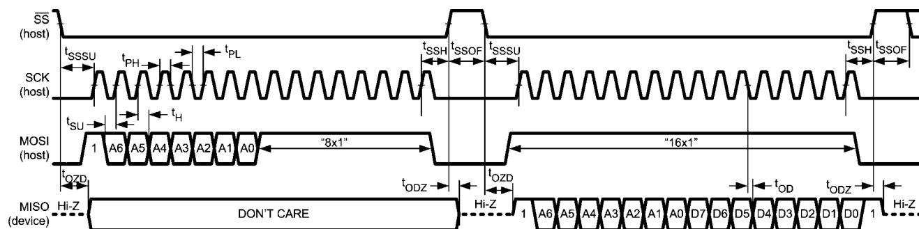
FIGURE 3. SPI Read
