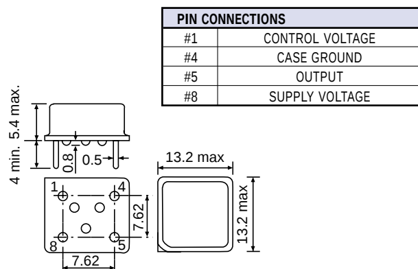
Figure 2) ECX-VXO-83 – Side, Bottom and Top views
