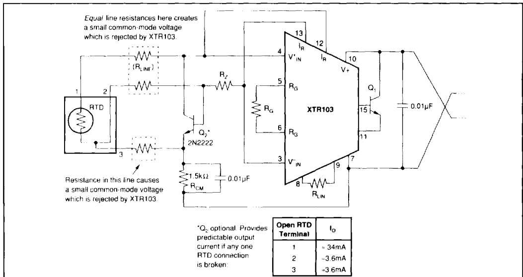
FIGURE 4. Three-Wire Connection for Remotely Located RTDs.
