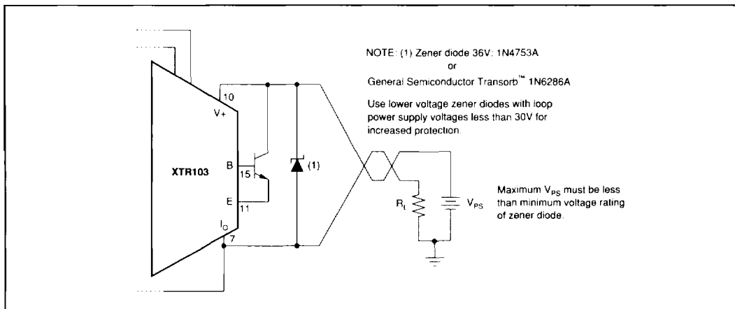
FIGURE 6. Over-Voltage Surge Protection.
