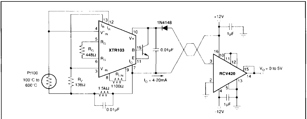
FIGURE 8. ±12V-Powered Transmitter/Receiver Loop.
