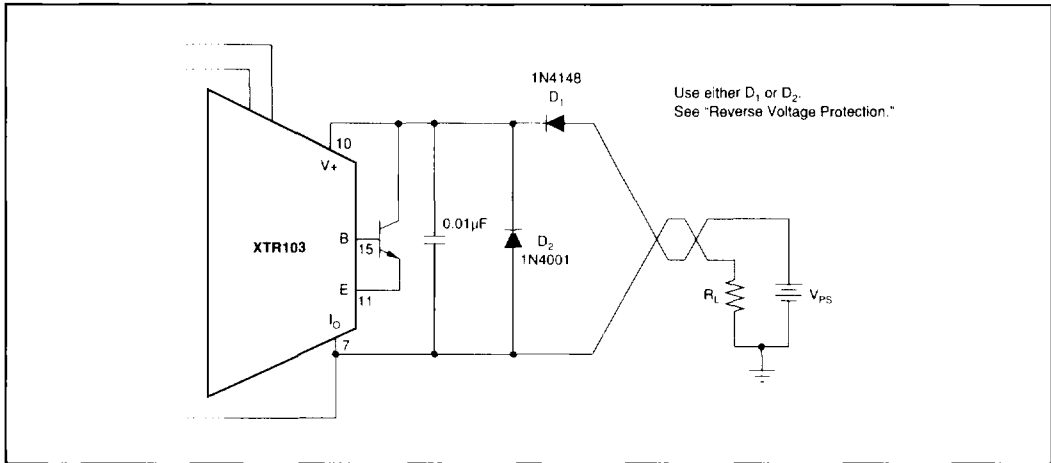
FIGURE 5. Reverse Voltage Protection.
