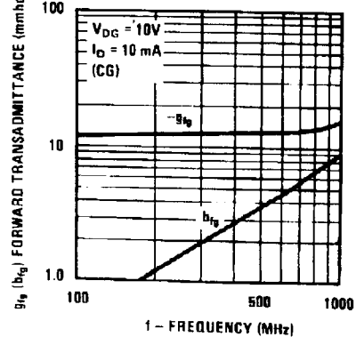
Forward Transmittance
