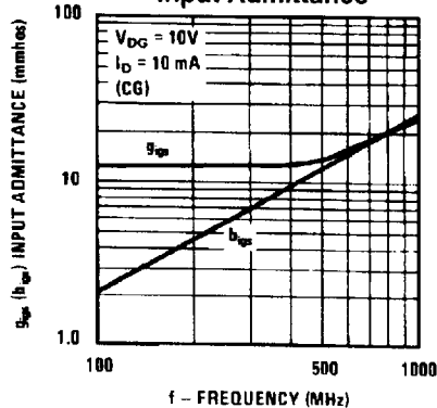
Input Admittance
