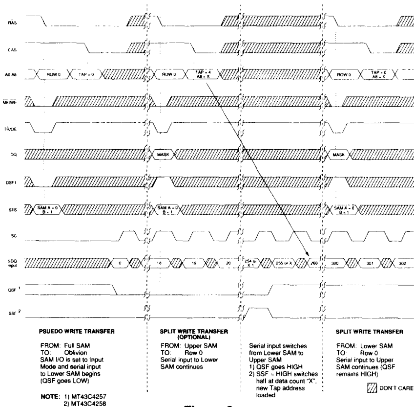
Figure 6 TYPICAL SPLIT-WRITE-TRANSFER INITIATION SEQUENCE
