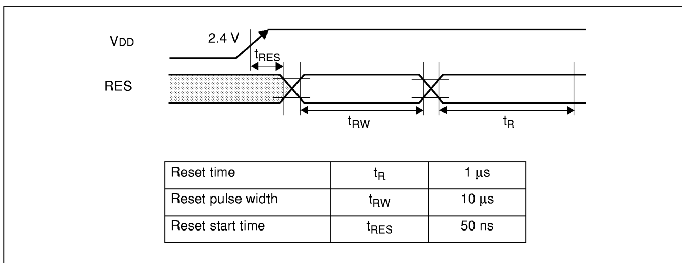
Figure 10. RESET Timing
