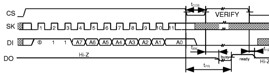
Figure 15 ERASE Timing (S-29330A)
