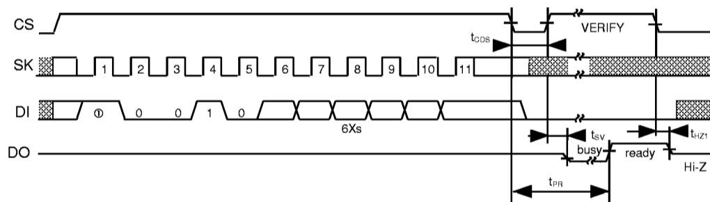
Figure 22 ERAL Timing (S-29220A)
