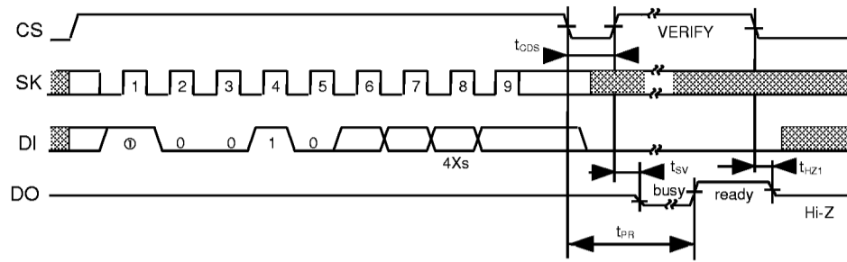
Figure 20 ERAL Timing (S-29130A)
