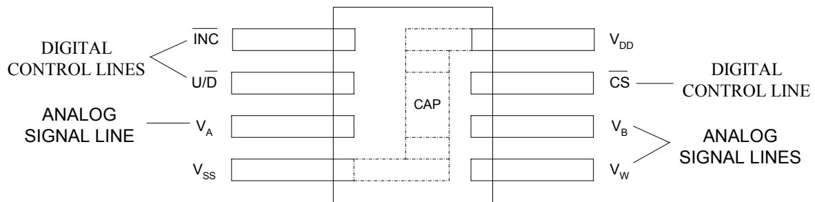
FIGURE 9 – WMS7170/1 LAYOUT
