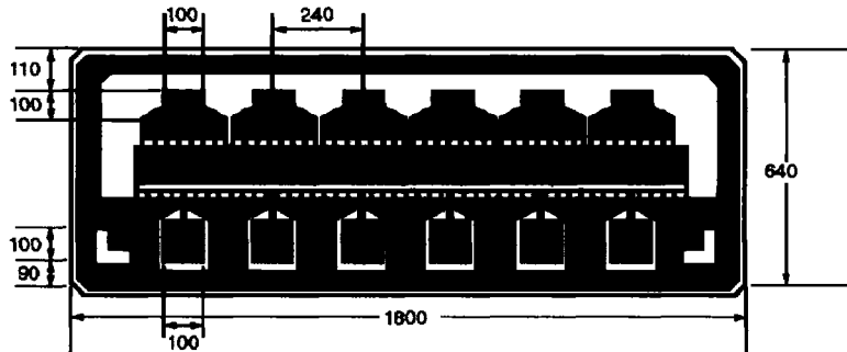
NE8500200 (CHIP) (Units in \mu\text{m} )
