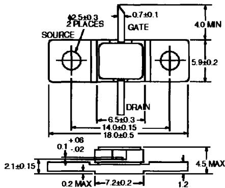
PACKAGE OUTLINE 95 (Units in mm)
