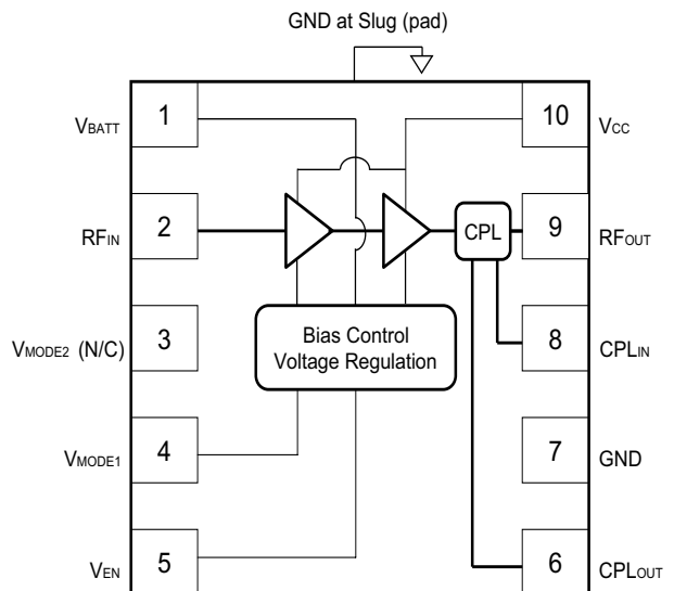
Figure 1: Block Diagram
