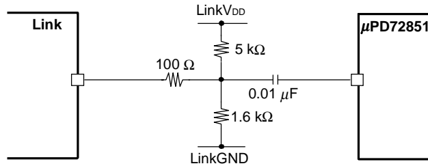
(b) Link-on Isolation Barrier Circuit
