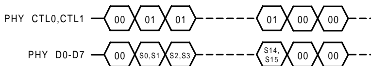
Figure 4-5. Status Timing
