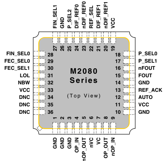
Figure 1: Pin Assignment
