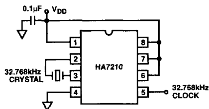
32.768kHz MICROPOWER CLOCK OSCILLATOR
