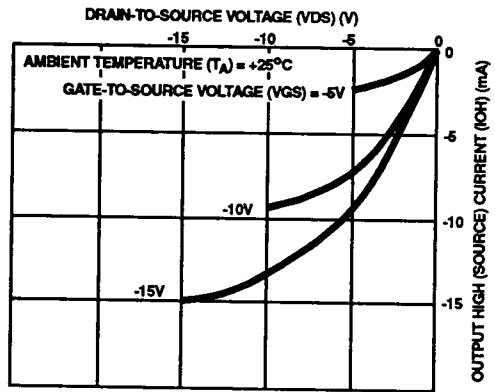
FIGURE 4. MINIMUM OUTPUT HIGH (SOURCE) CURRENT CHARACTERISTICS
