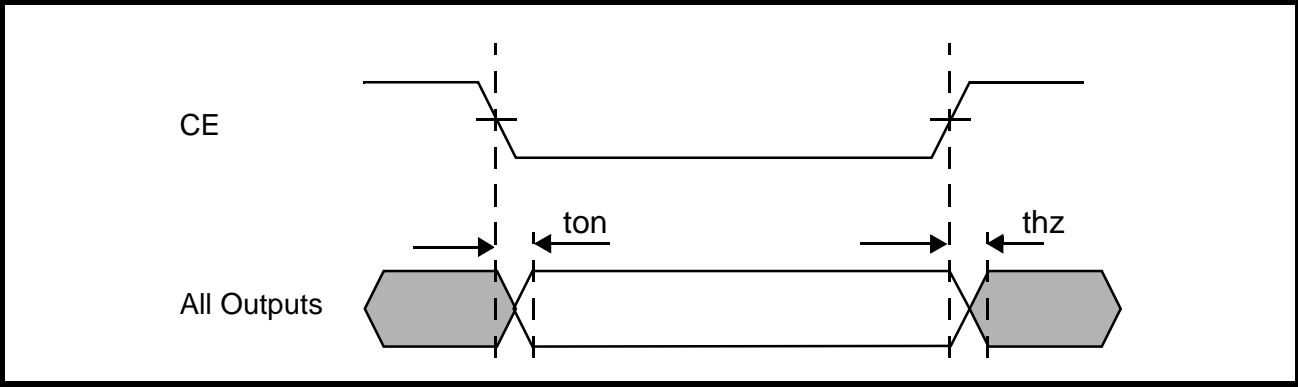
Figure 11: Chip Enable Timing (Refer to Table 9)
