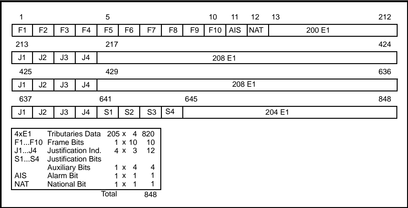
Figure 3: E2 Frame
