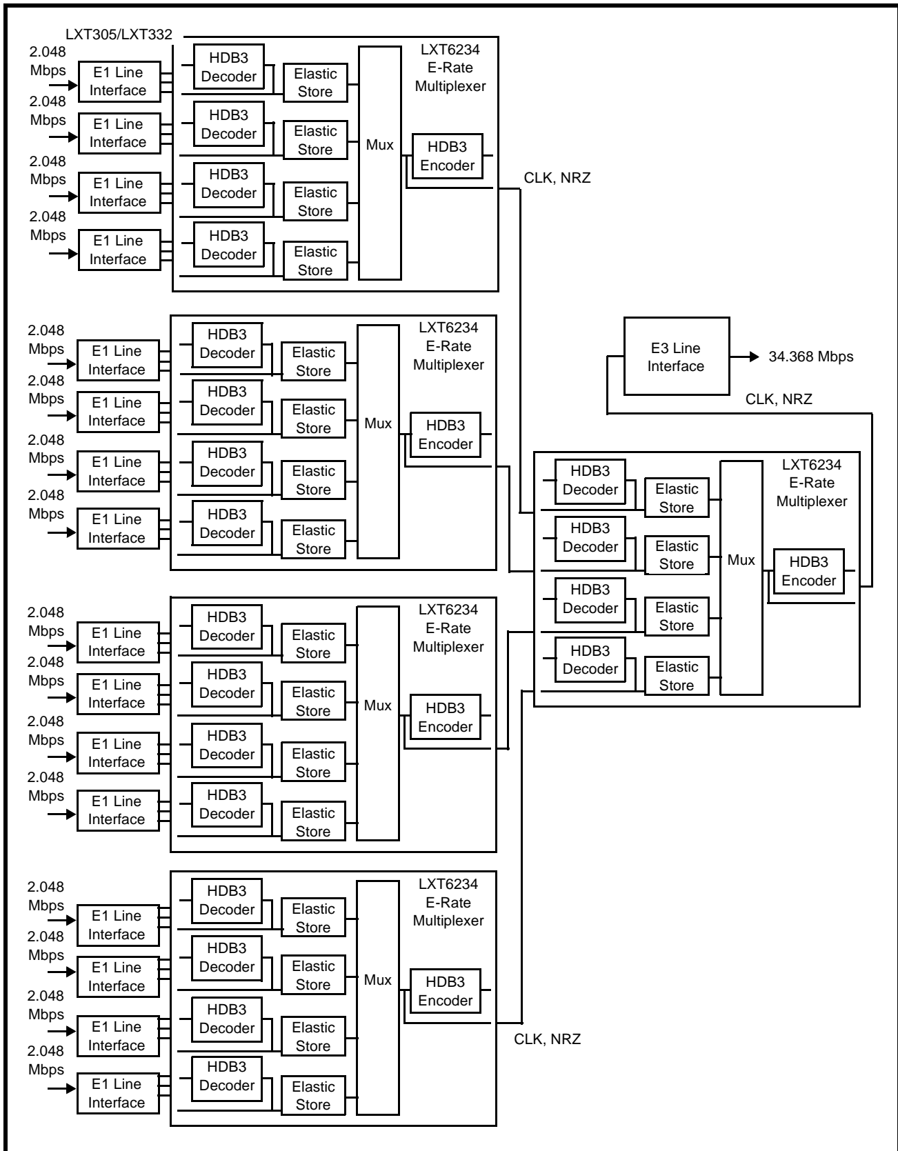
Figure 6: E1/E3 Multiplexer
