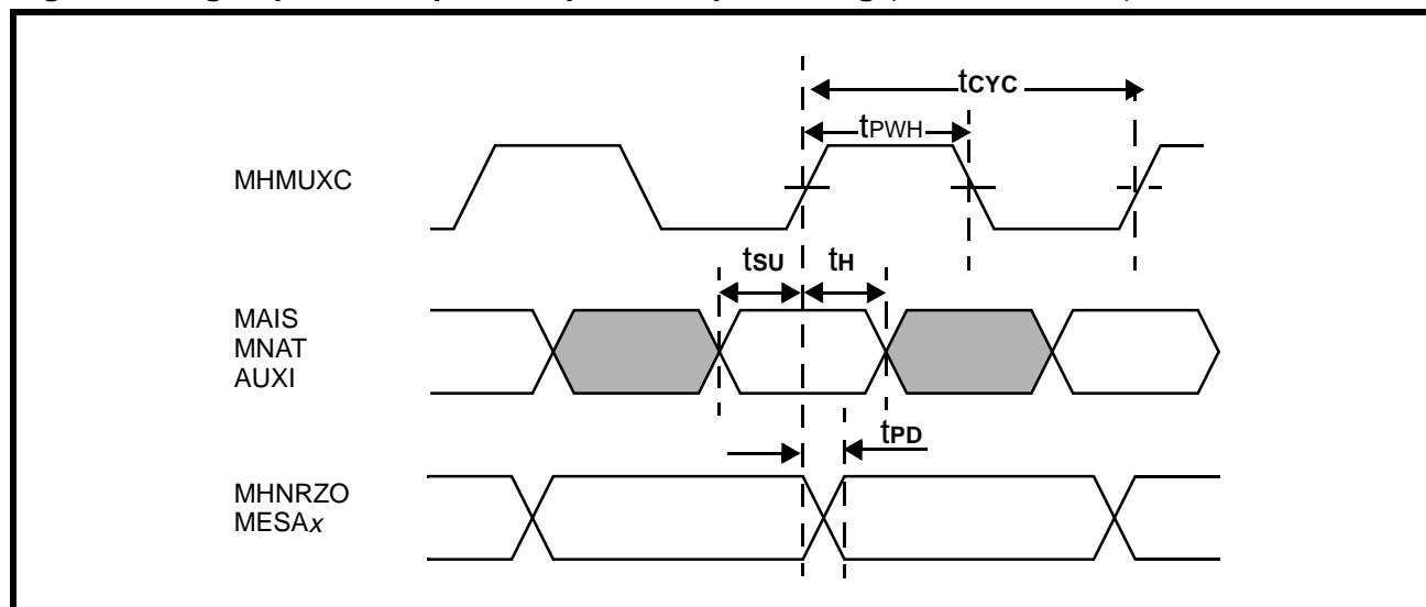
Figure 9: High Speed Multiplexer Input & Output Timing (Refer to Table 7)
