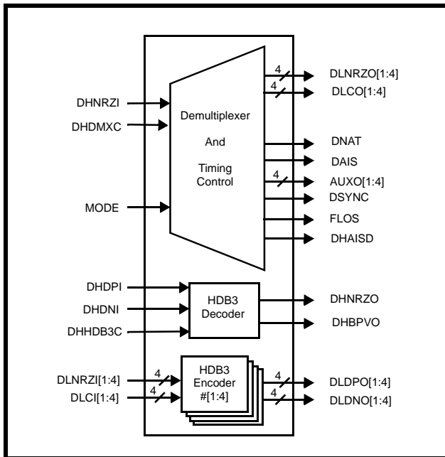
Figure 5: Demultiplexer Side Block Diagram
