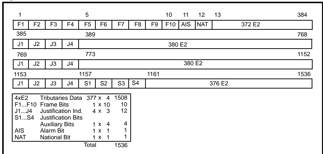
Figure 4: E3 Frame
