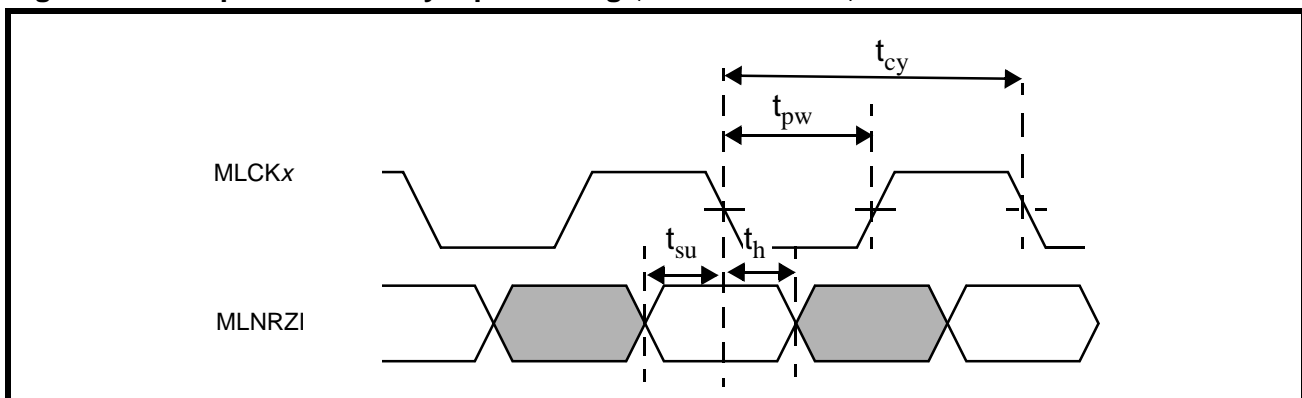
Figure 8: Multiplexer Tributary Input Timing (Refer to Table 6)
