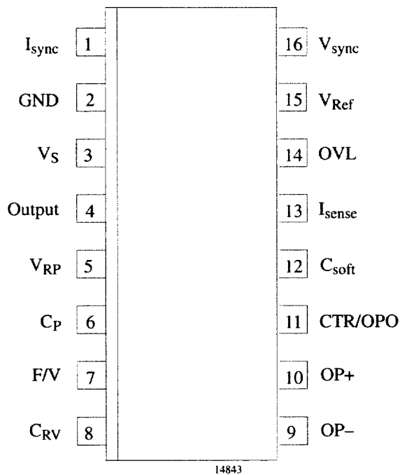
Figure 4. Pinning SO16
