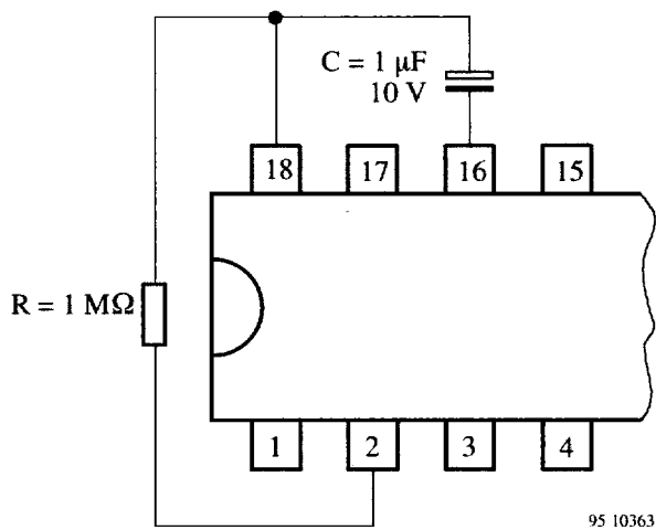
Figure 7. Operation delay
