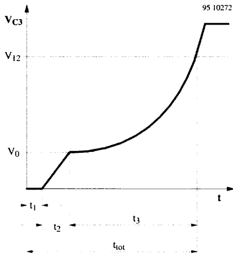
Figure 6. Soft-start
