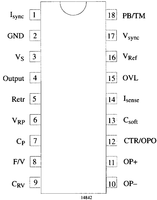
Figure 3. Pinning DIP18
