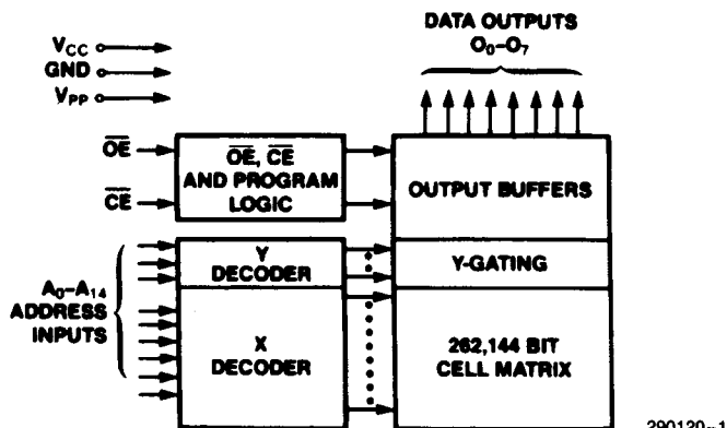
Figure 1. Block Diagram
