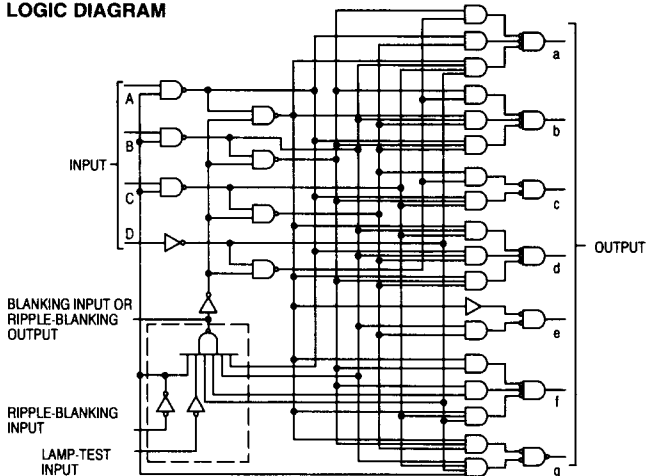
LOGIC DIAGRAM
