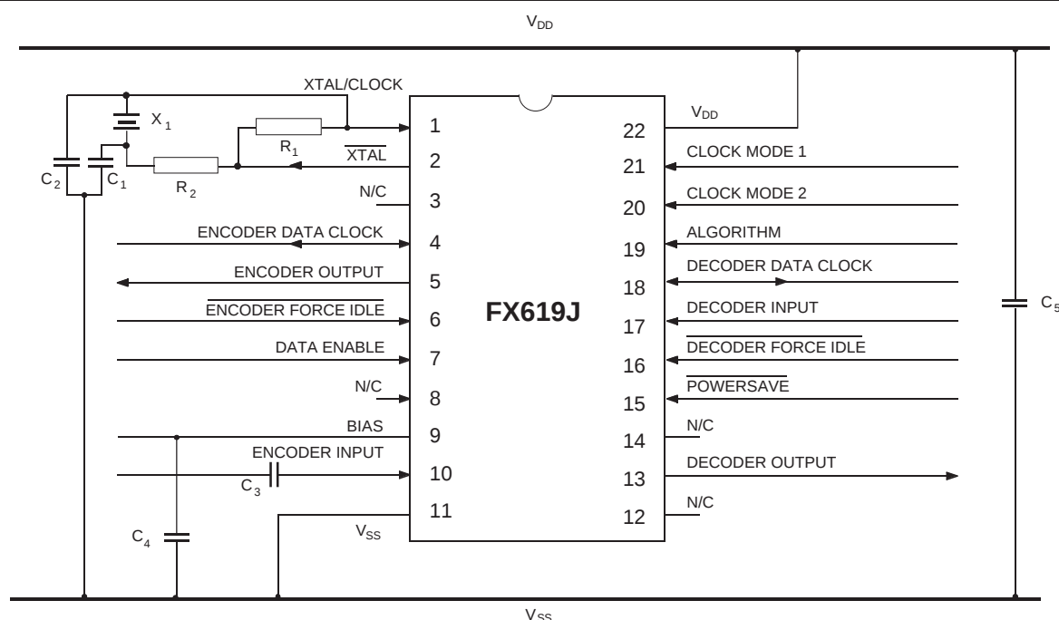
Fig.3 Recommended External Components
