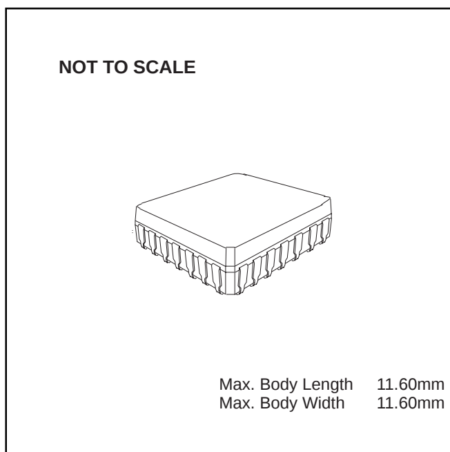
FX619M1 28-lead ceramic leaded chip carrier (M1)
