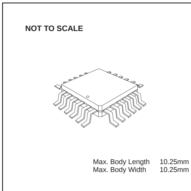
FX619L1 24-pin quad plastic encapsulated bent and cropped (LG)
