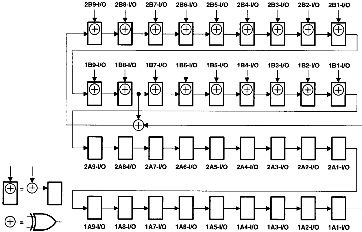
Figure 9. 36-Bit PSA Configuration (1OEAB = 2OEAB = 0, 1OEBA = 2OEBA = 0)
