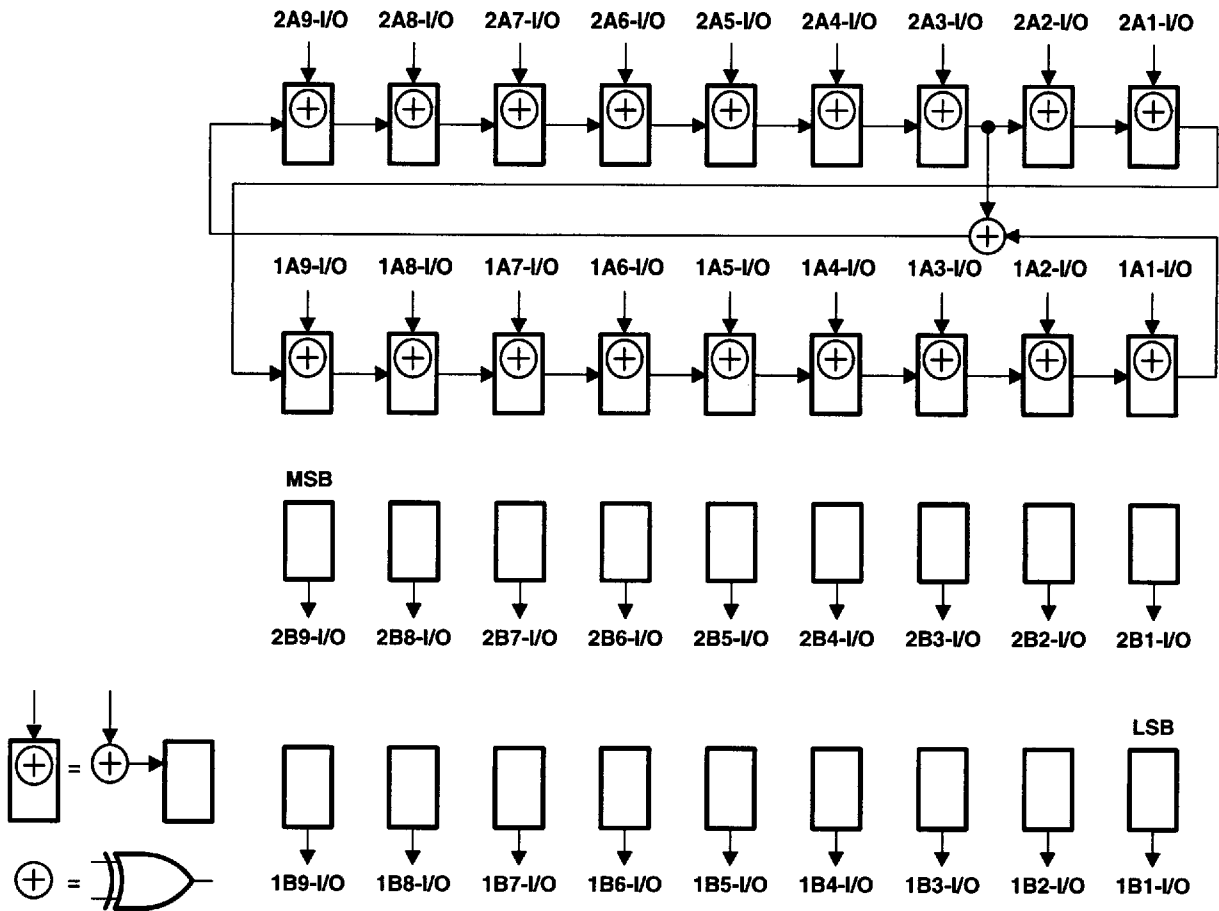
Figure 12. 18-Bit PSA/COUNT Configuration (1OEAB = 2OEAB = 1, 1OEBA = 2OEBA = 1)
