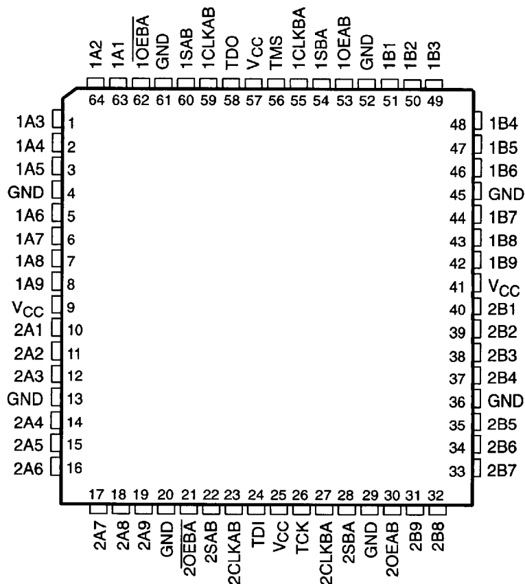
SN74LVTH18652A, SN74LVTH182652A . . . PM PACKAGE (TOP VIEW)
