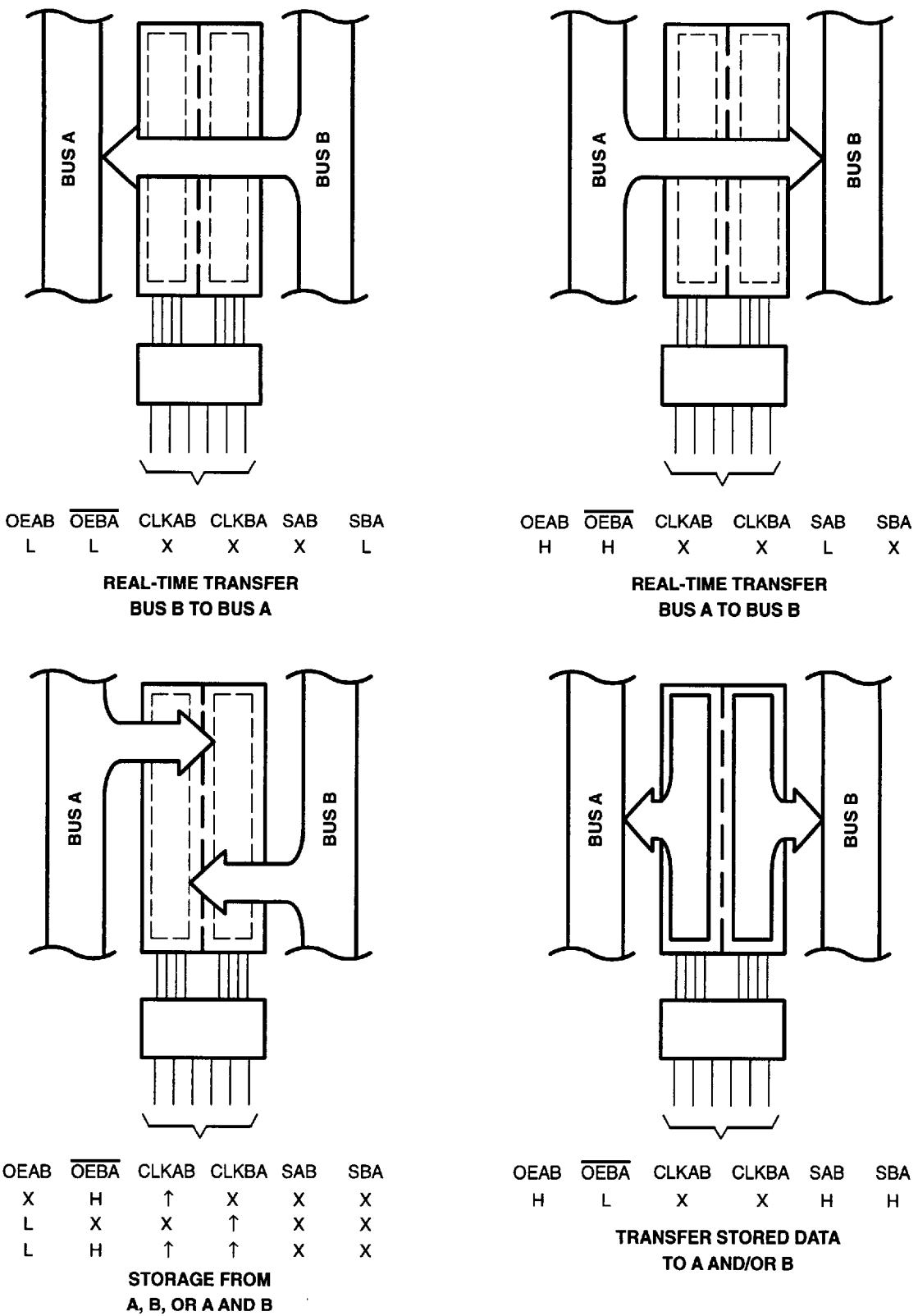
Figure 1. Bus-Management Functions
