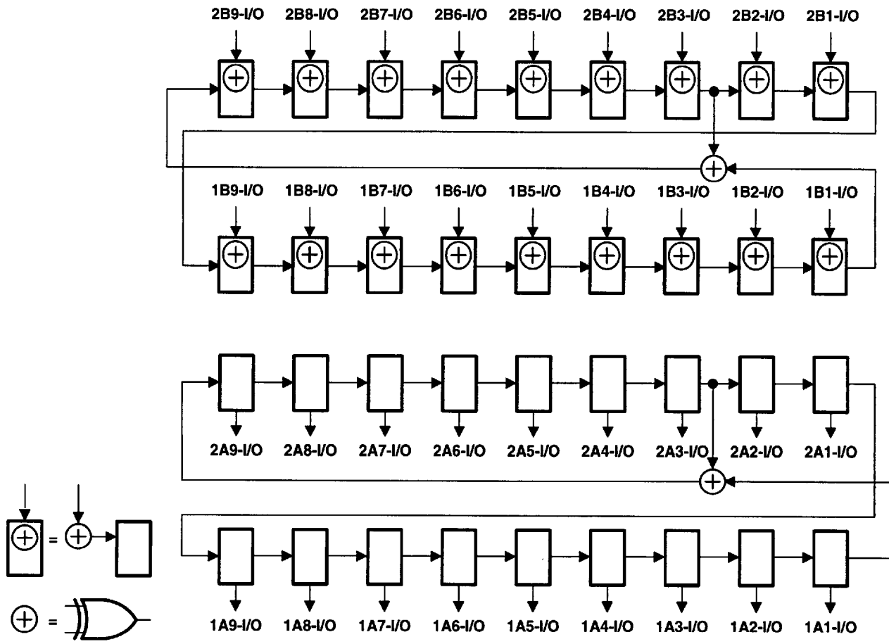
Figure 11. 18-Bit PSA/PRPG Configuration (1OEAB = 2OEAB = 0, 1OEBA = 2OEBA = 0)
