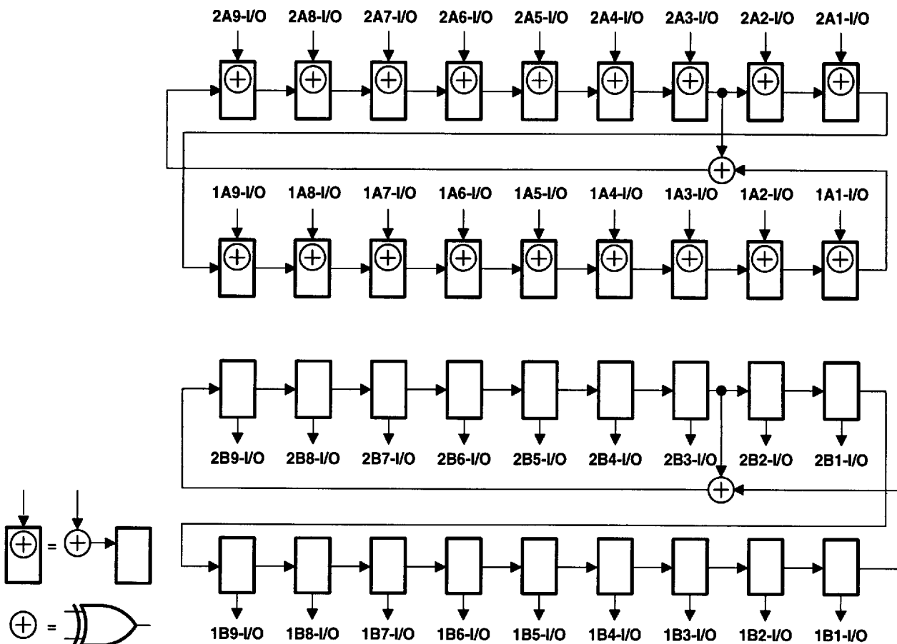
Figure 10. 18-Bit PSA/PRPG Configuration (1OEAB = 2OEAB = 1, 1OEBA = 2OEBA = 1)
