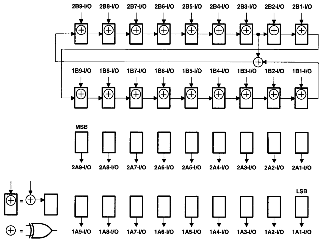
Figure 13. 18-Bit PSA/COUNT Configuration (1OEAB = 2OEAB = 0, 1OEBA = 2OEBA = 0)
