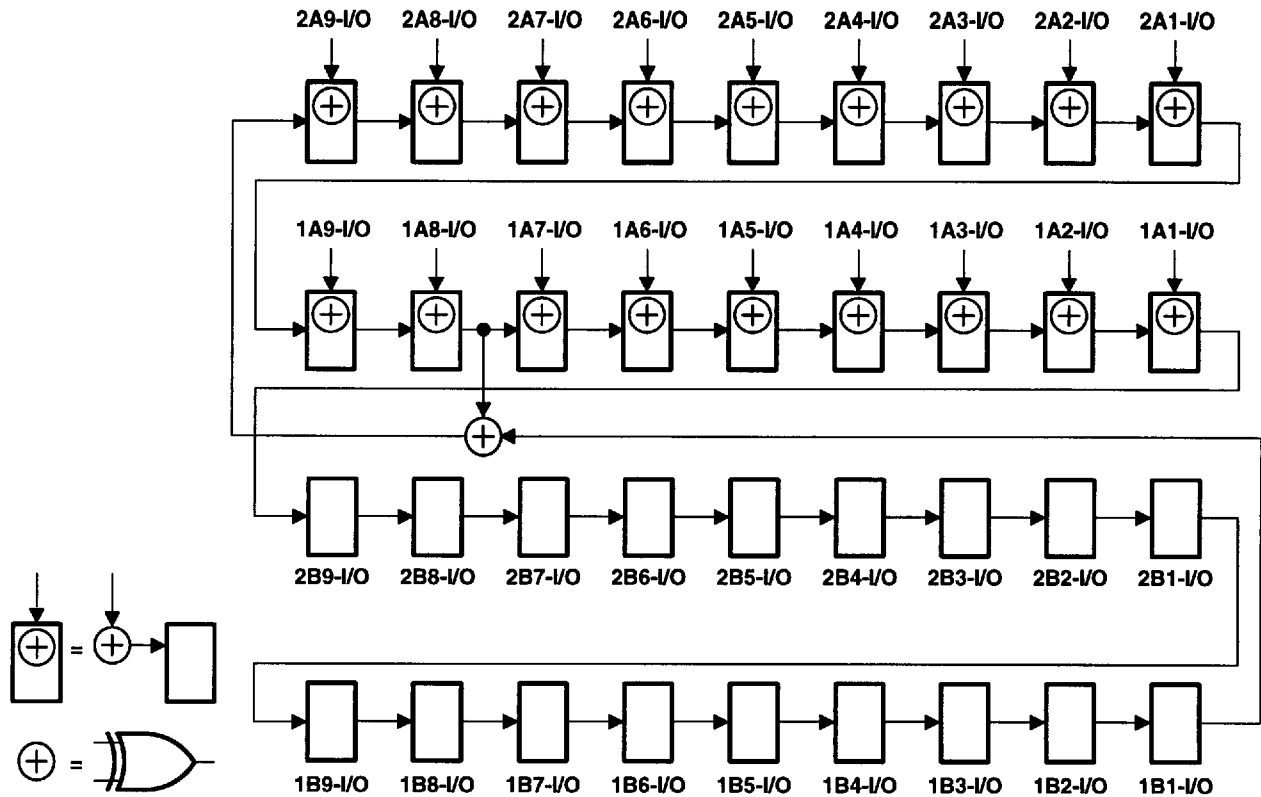
Figure 8. 36-Bit PSA Configuration (1OEAB = 2OEAB = 1, 1OEBA = 2OEBA = 1)
