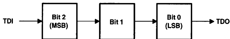
Figure 4. Boundary-Control Register Order of Scan
