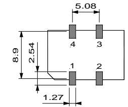
PC board footprint
