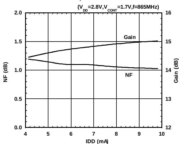
NF, Gain vs. IDD
