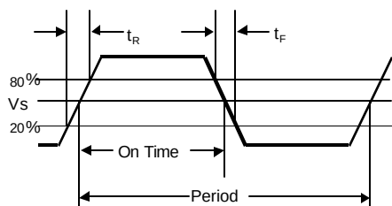
Figure 7. Output Waveform
