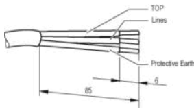
Fig. 1: Recommended stripping lengths in mm
