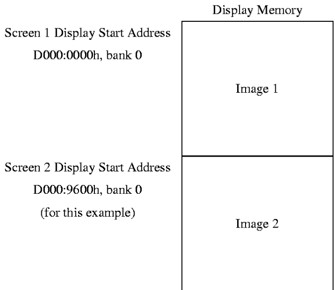
Figure 16: Memory Map For Split Screen
