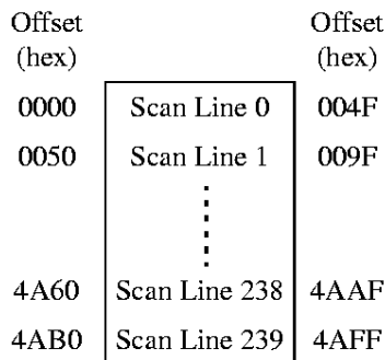
Figure 10: Memory Map Example For 320 x 240 LCD Panel With 4 Colors/Gray Shades
