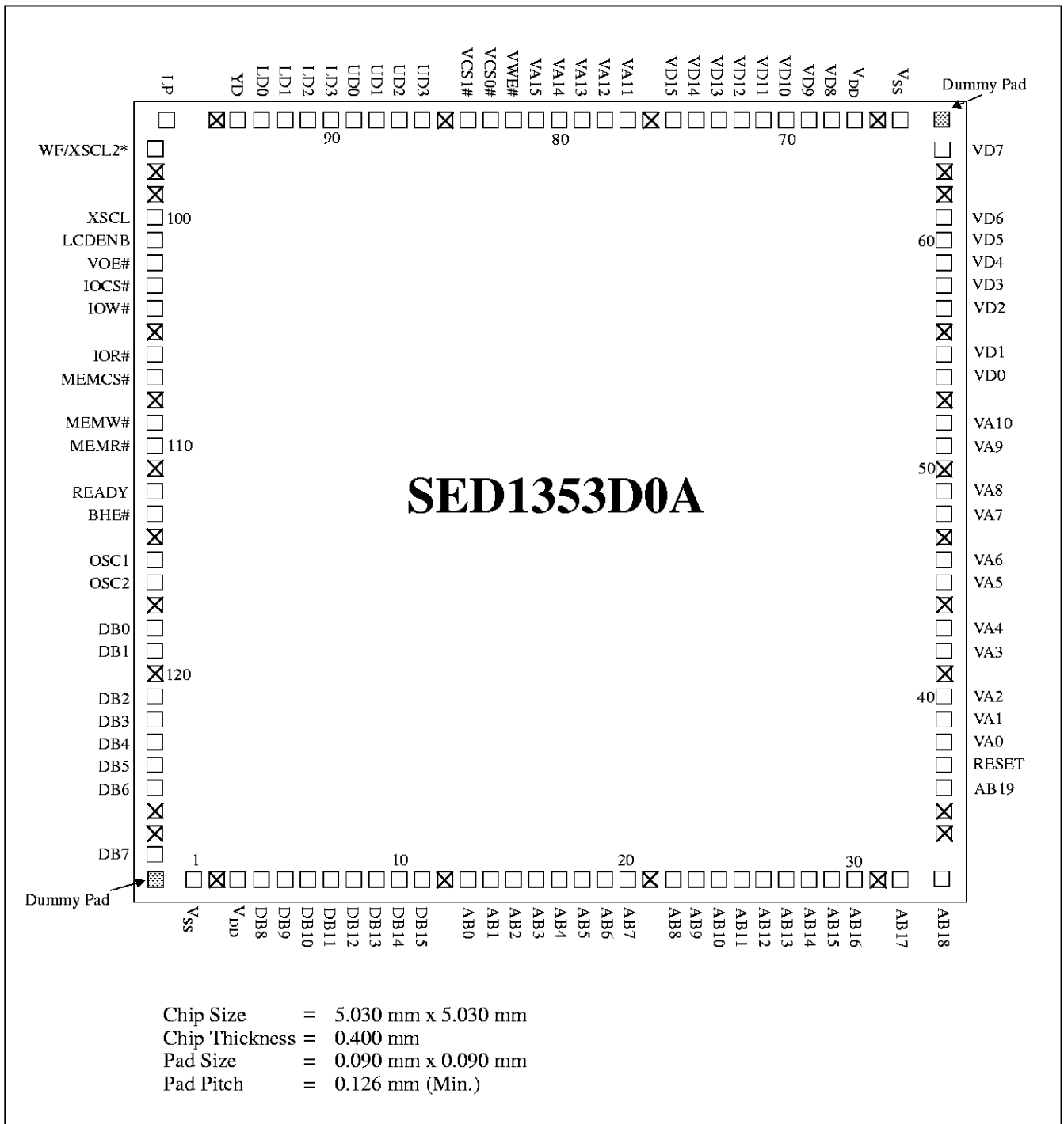
Figure 9: SED1353D0A Pad Diagram
