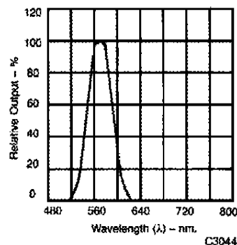
Fig. 2. Spectral Response
