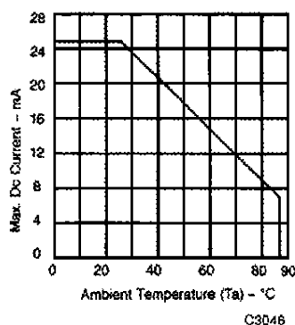
Fig. 4. Maximum Allowable DC Current Per Segment vs. Ambient Temperature
