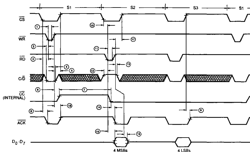
MODE 3 TIMING DIAGRAM
