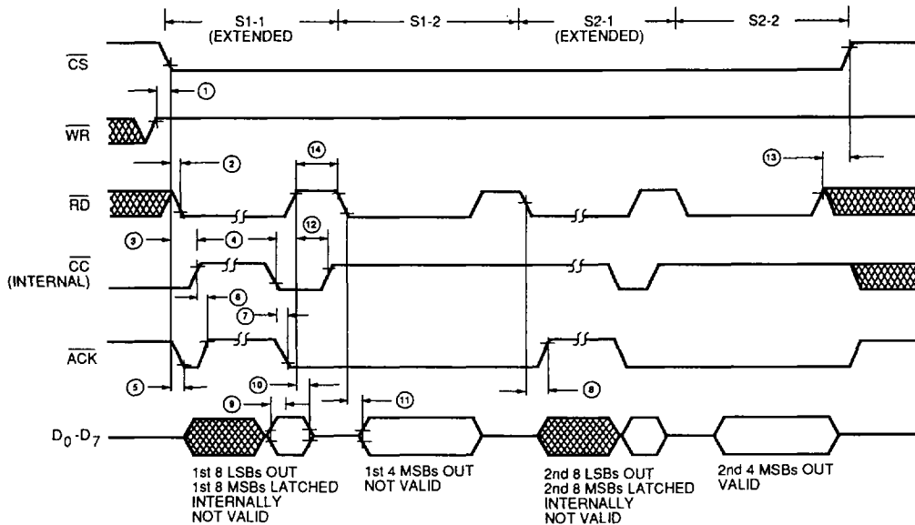
MODE 2 TIMING DIAGRAM
