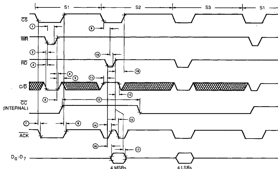
MODE 0 TIMING DIAGRAM
