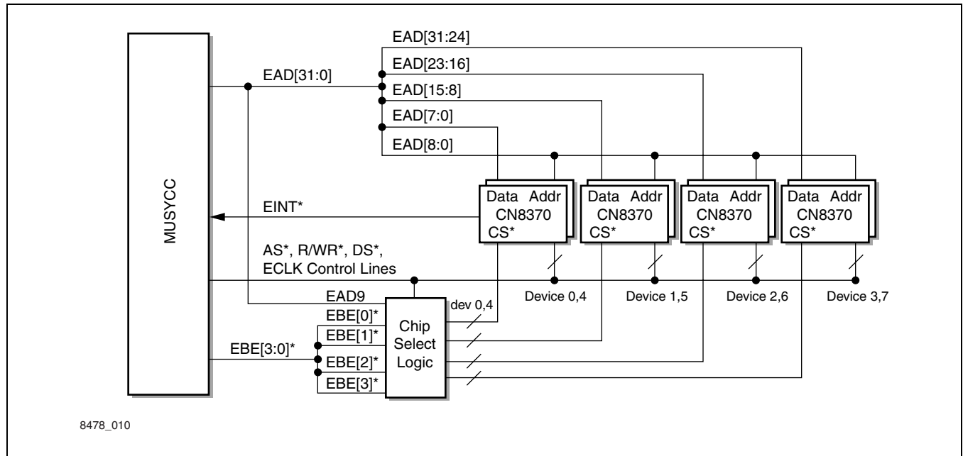
Figure 3-4. EBUS Connection, Non-multiplexed Address/Data, 8 Framers, No MPU
