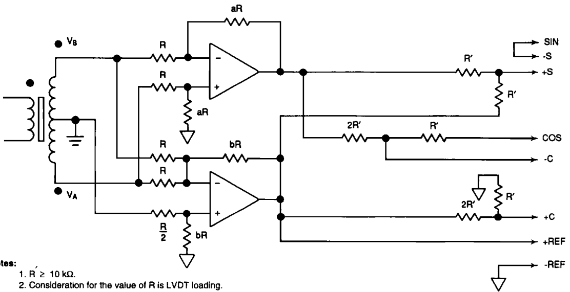
FIGURE 11B. 3-WIRE LVDT DIRECT INPUT
