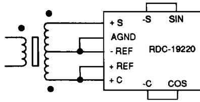
FIGURE 11B. 3-WIRE LVDT DIRECT INPUT
