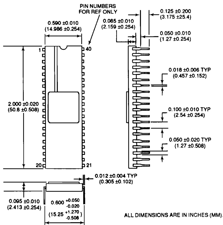
FIGURE 18. RDC-19220/RDC-19223 (40 PIN DDIP) CERAMIC PACKAGE MECHANICAL OUTLINE
