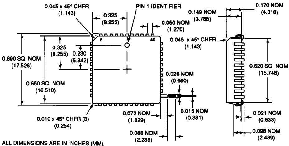
FIGURE 19. RDC-19222 (44 PIN PLASTIC J-LEAD) MECHANICAL OUTLINE
