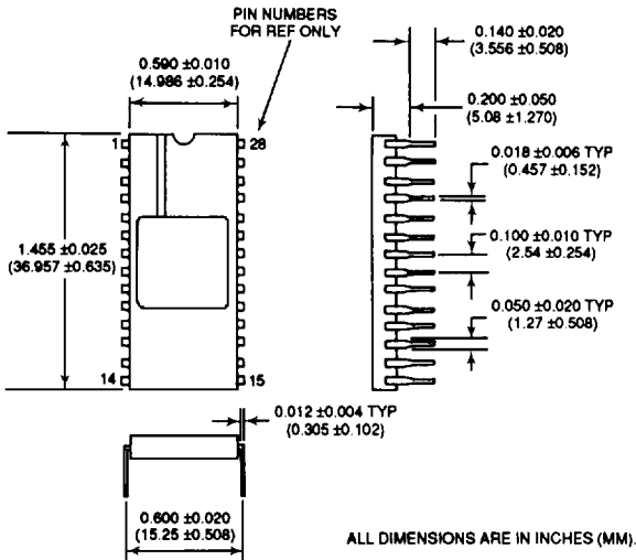
FIGURE 21. RDC-19221 (28 PIN CERAMIC DDIP) MECHANICAL OUTLINE
