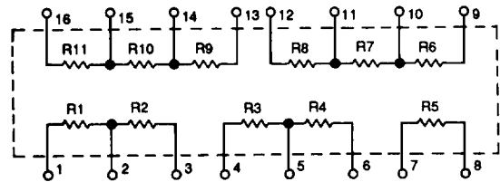
FIGURE 23. DDC-49530 AND DDC-49590 LAYOUT AND RESISTOR VALUES (See TABLE 10.)
