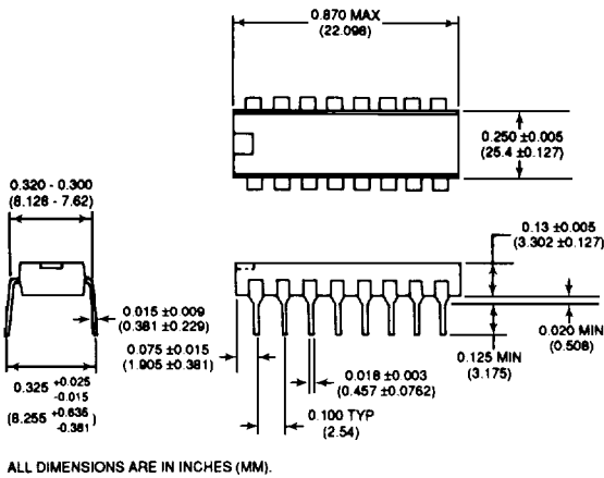
FIGURE 22. 16 PIN DIP THIN-FILM RESISTOR NETWORK MECHANICAL OUTLINE (DDC-49530, DDC-49590)
