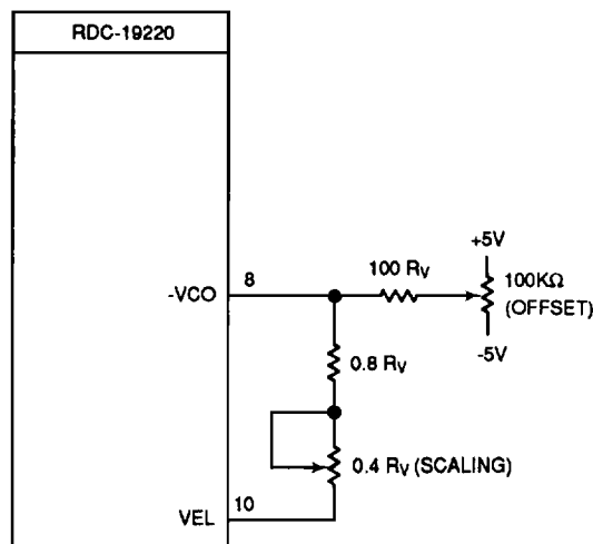
FIGURE 9. VELOCITY TRIMMING
