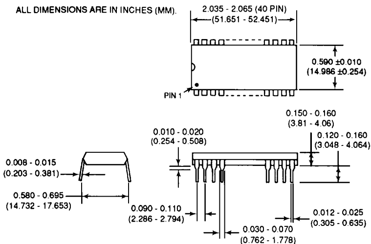
FIGURE 17. RDC-19220/RDC-19223 (40 PIN DDIP) PLASTIC PACKAGE MECHANICAL OUTLINE
