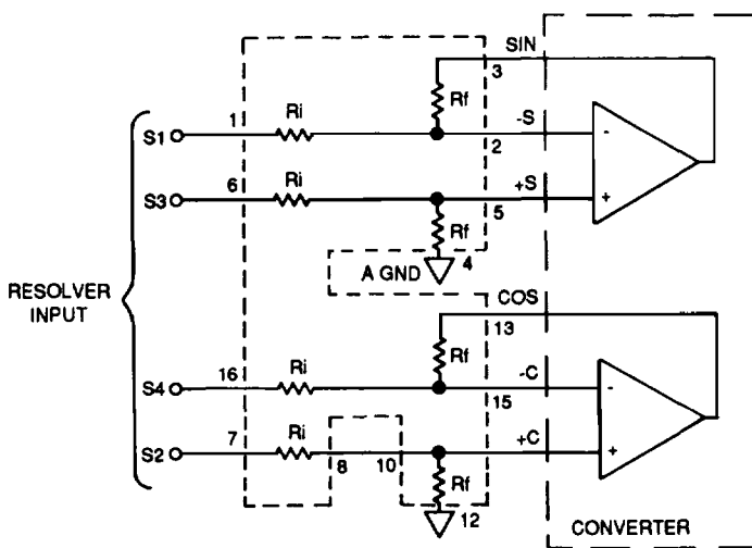
FIGURE 7A. DIFFERENTIAL RESOLVER INPUT
