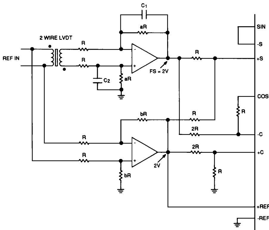
FIGURE 11A. 2-WIRE LVDT DIRECT INPUT
