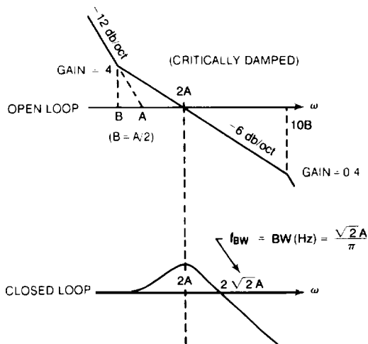
FIGURE 4. BODE PLOTS
