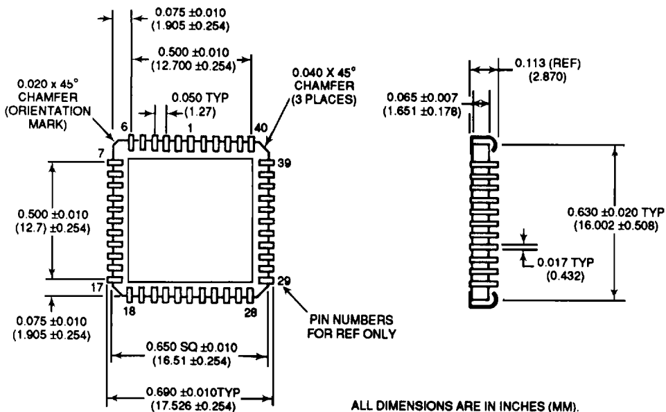
FIGURE 20. RDC-19222 (44 PIN CERAMIC J-LEAD) MECHANICAL OUTLINE
