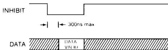
FIGURE 12. INHIBIT TIMING
