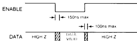
FIGURE 13. ENABLE TIMING
