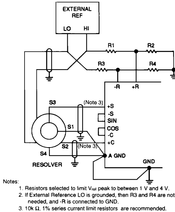
FIGURE 5. TYPICAL HOOK-UP, 2V RESOLVER, DIRECT INPUT
