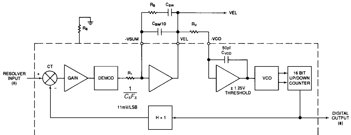
FIGURE 2. TRANSFER FUNCTION BLOCK DIAGRAM #1
