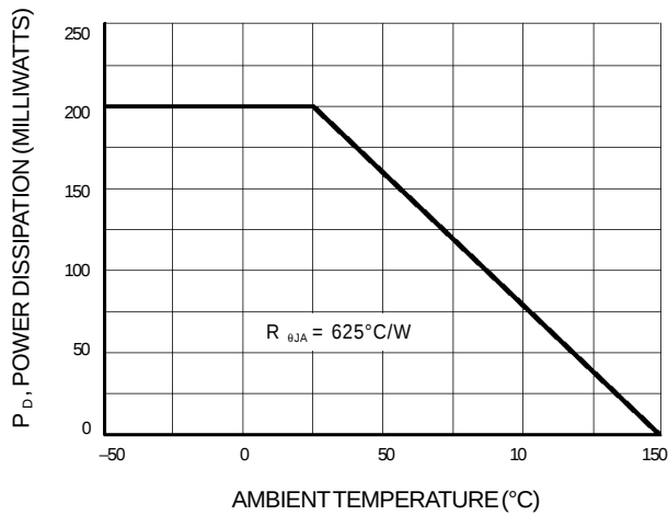
Figure 1. Derating Curve
