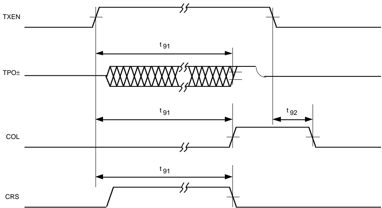
Figure 25. Jabber Timing
